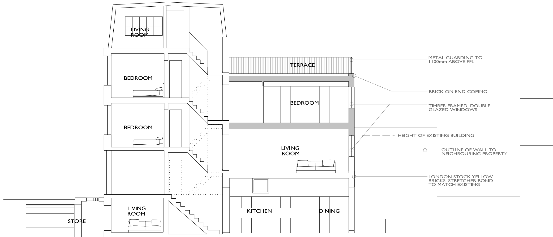
SECTION B-B
