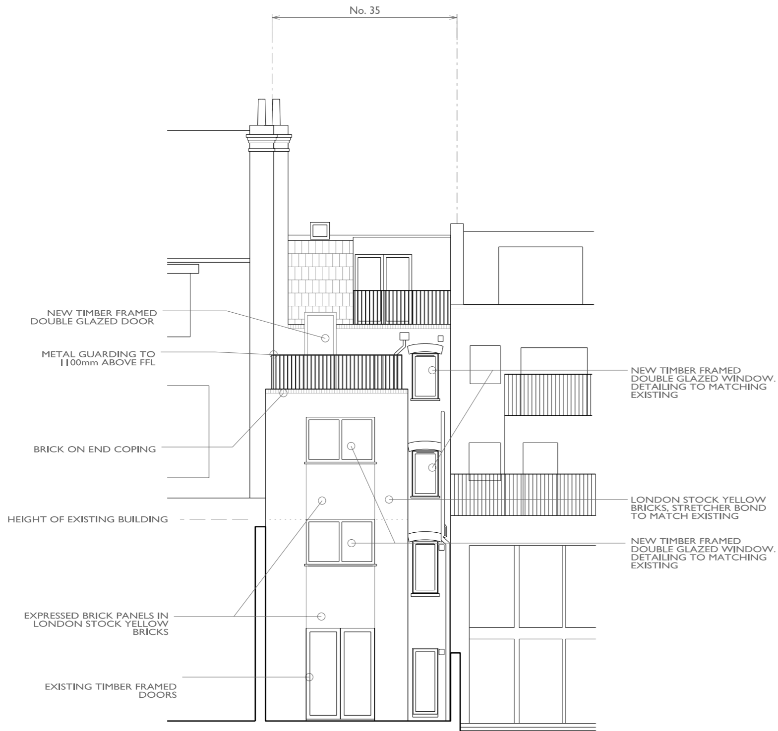
REAR ELEVATION
