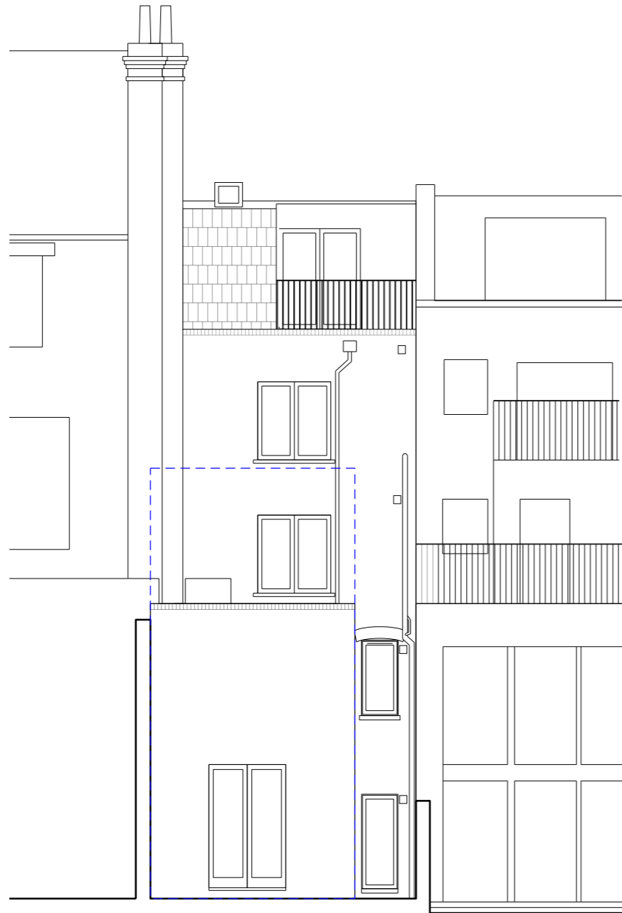
REAR ELEVATION
