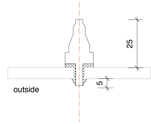
SECTION THROUGH GLAZING BEAD SCALE 1:1 @ A3
