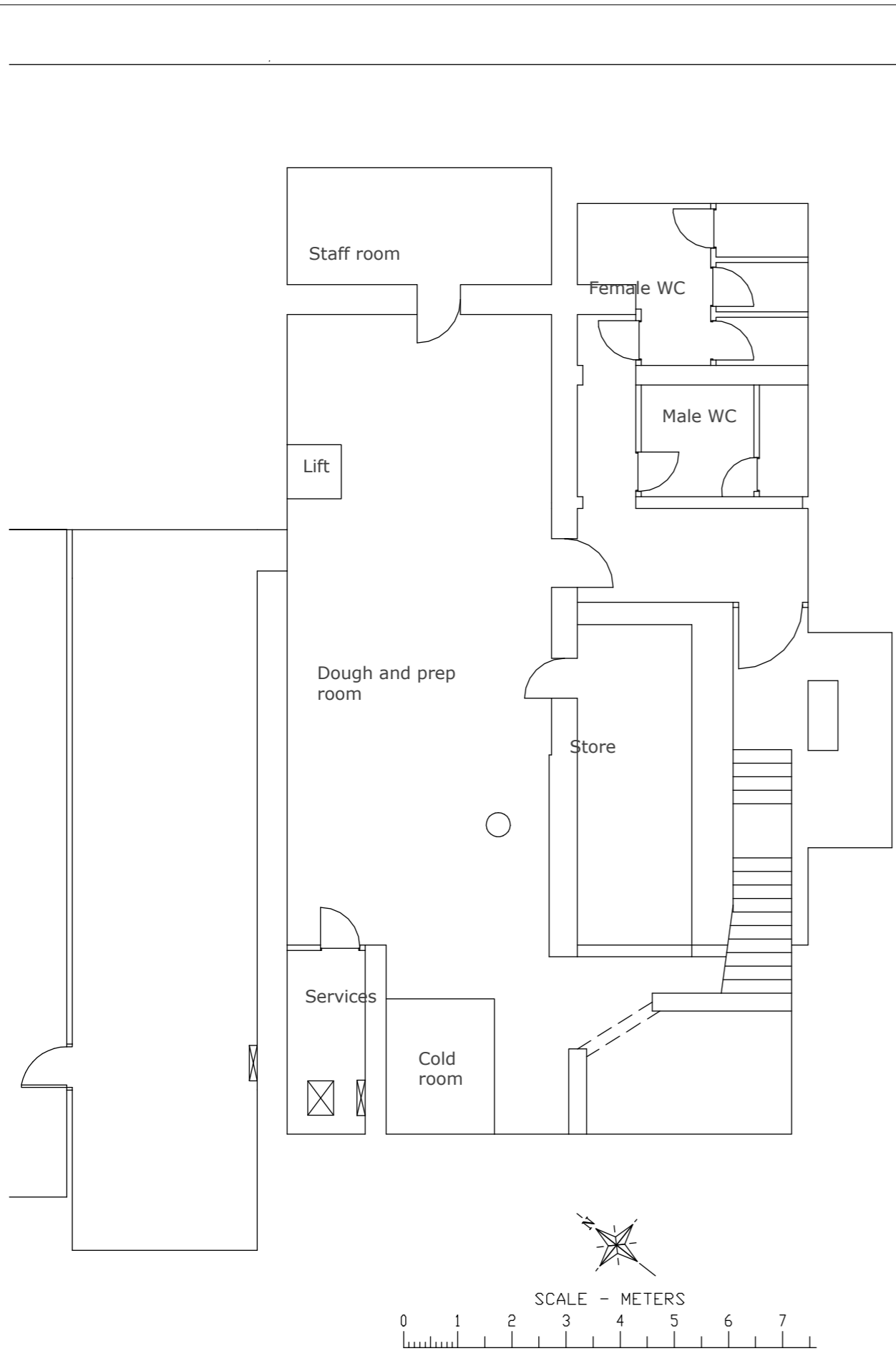
BASEMENT PLAN
