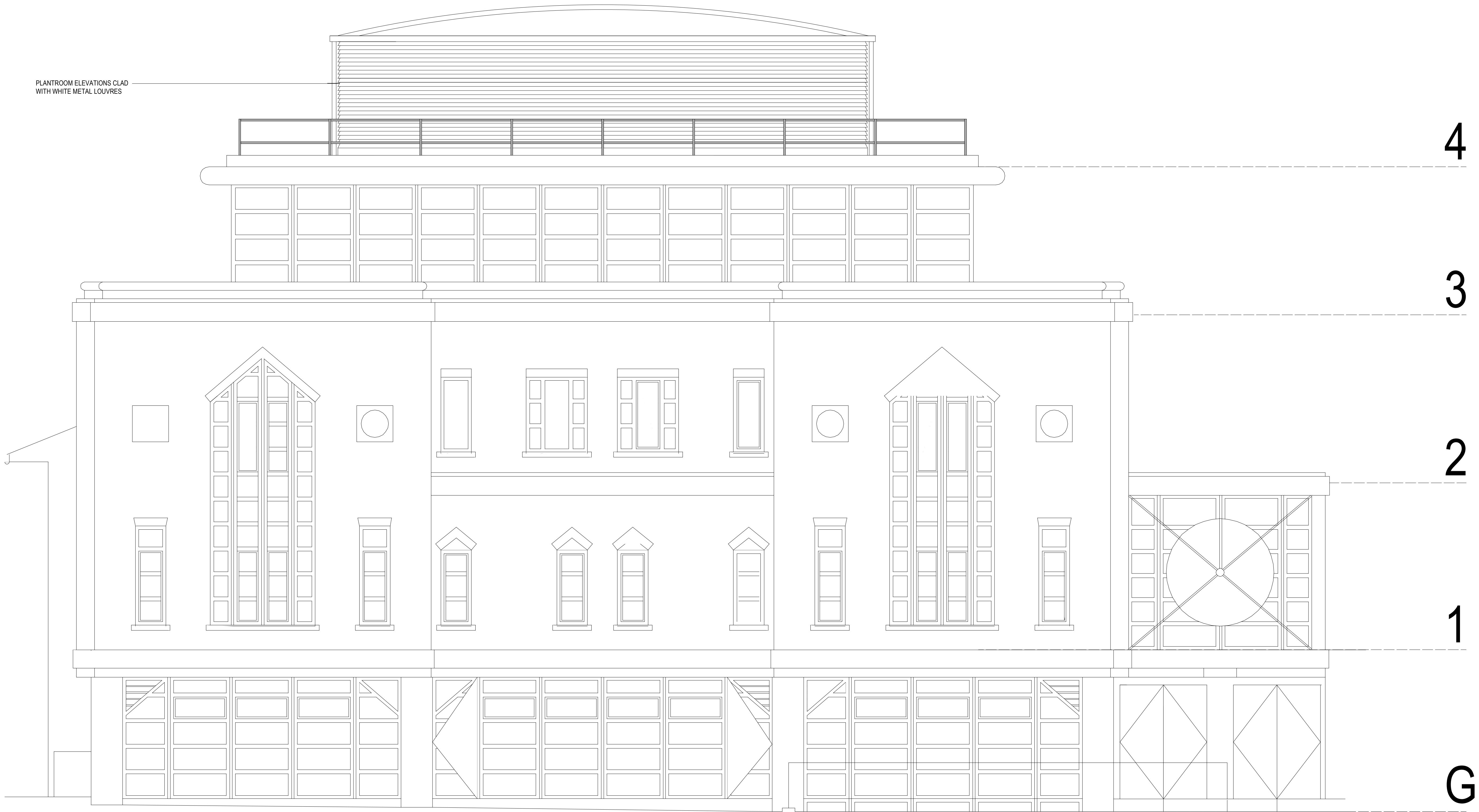
EXTERNAL ELEVATION MACKLIN STREET
