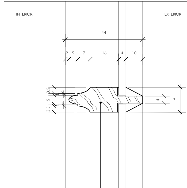
WINDOW SECTION THRU' GLAZING BAR (1:1)
