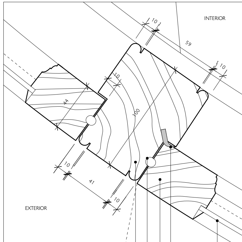
WINDOW DETAIL PLAN AT COLUMN (1:2)
