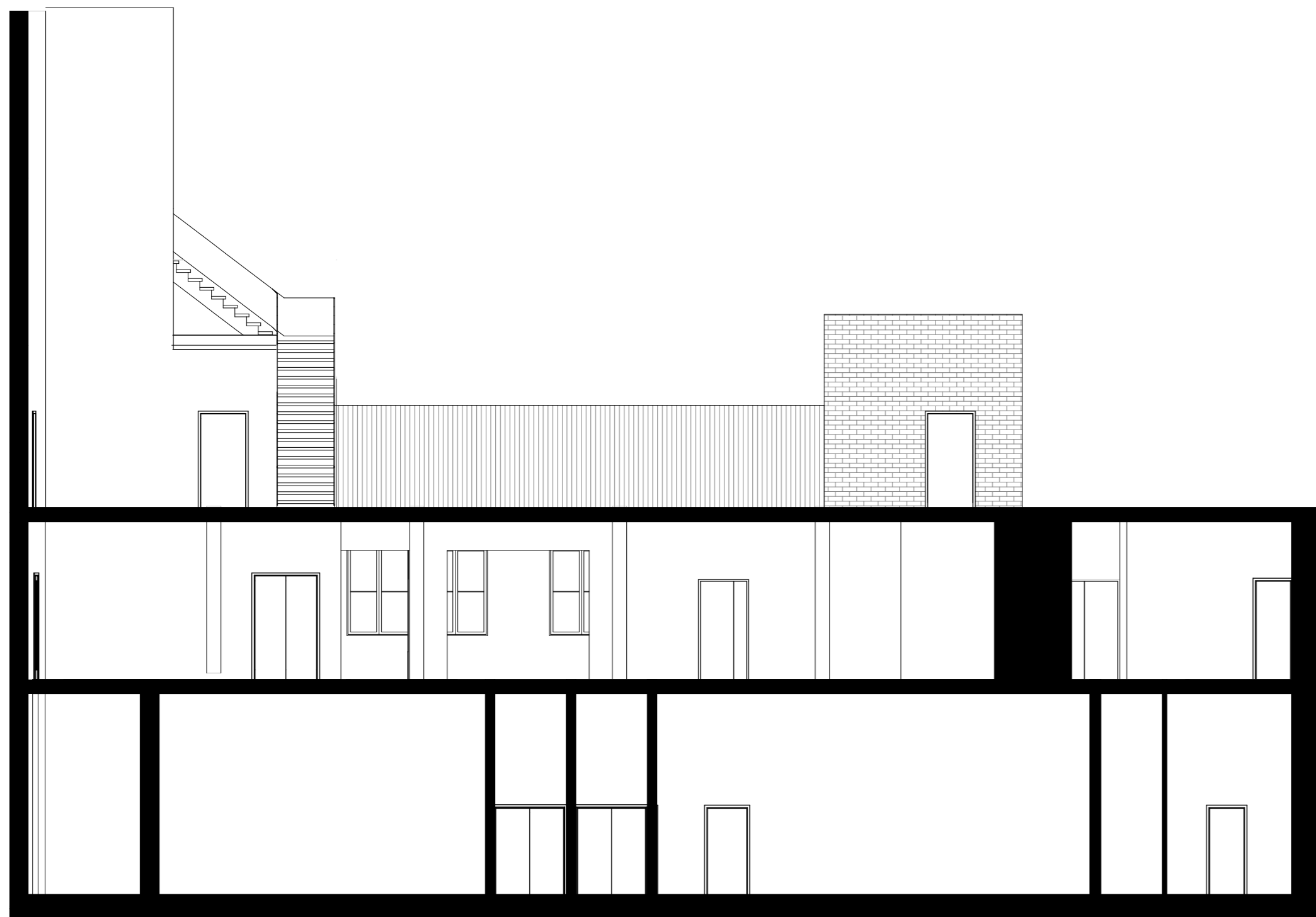
East elevation
