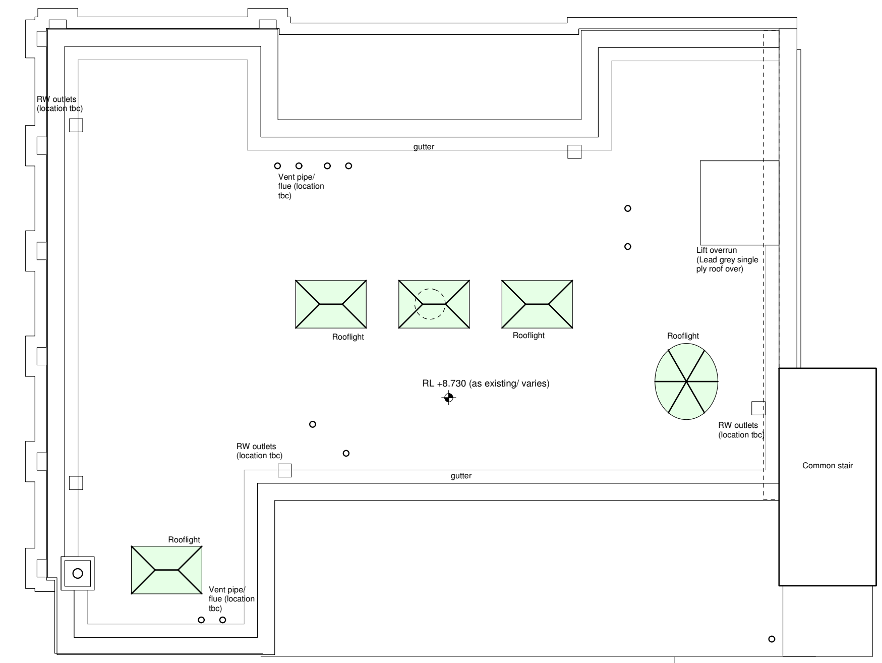
Proposed Roof Plan (1:100)
