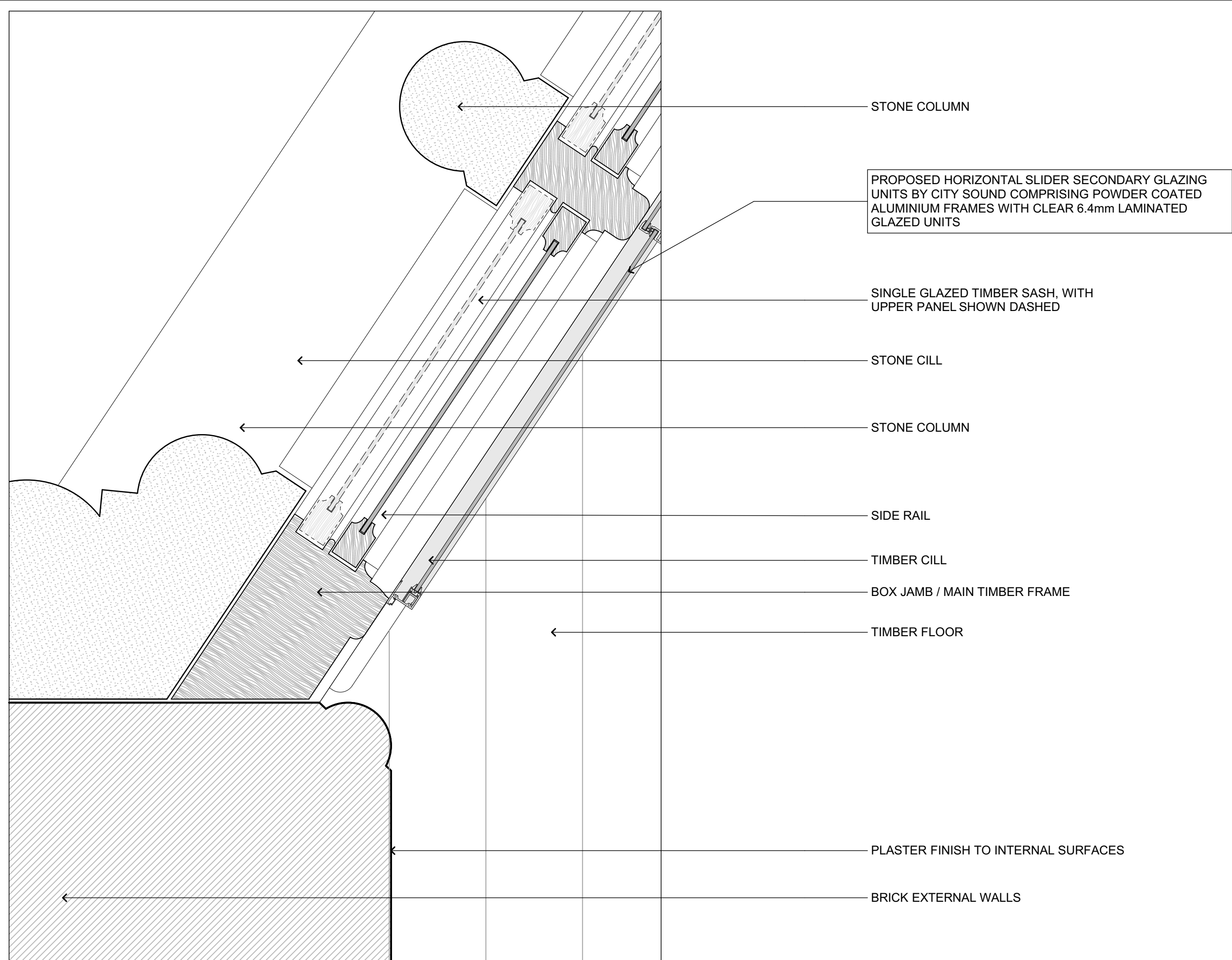
1 PROPOSED SIDE PANEL JAMB DETAIL
