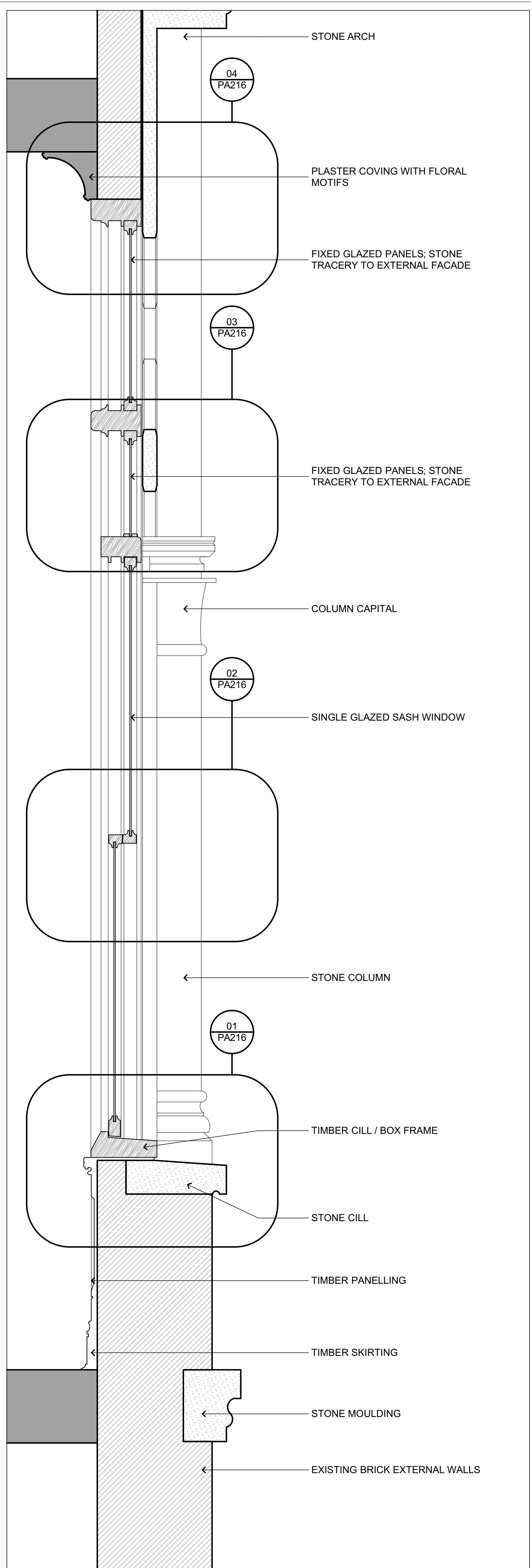
SECTION THROUGH EXISTING BAY WINDOW
