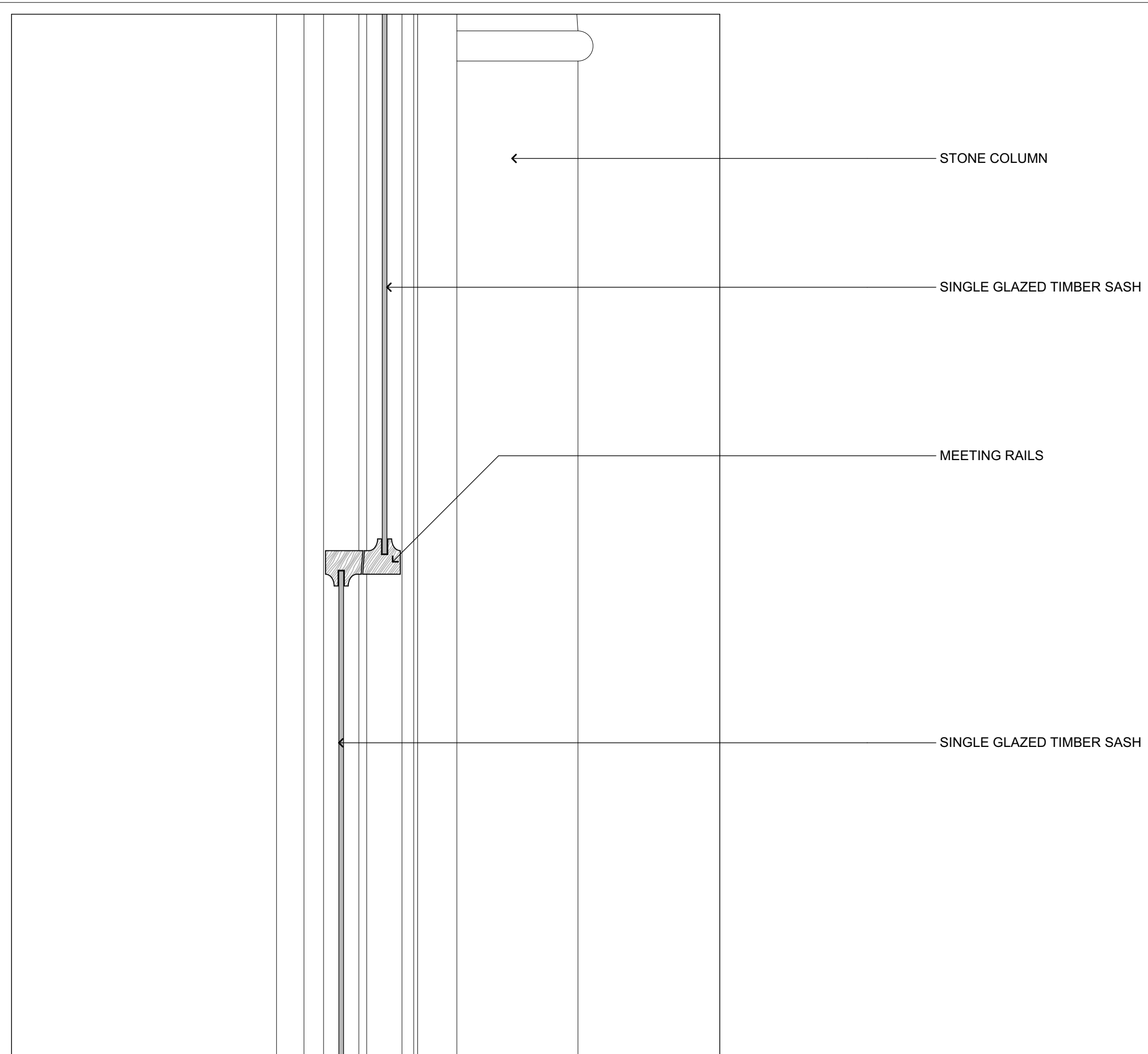
SECTIONAL DETAIL THROUGH MEETING RAIL
