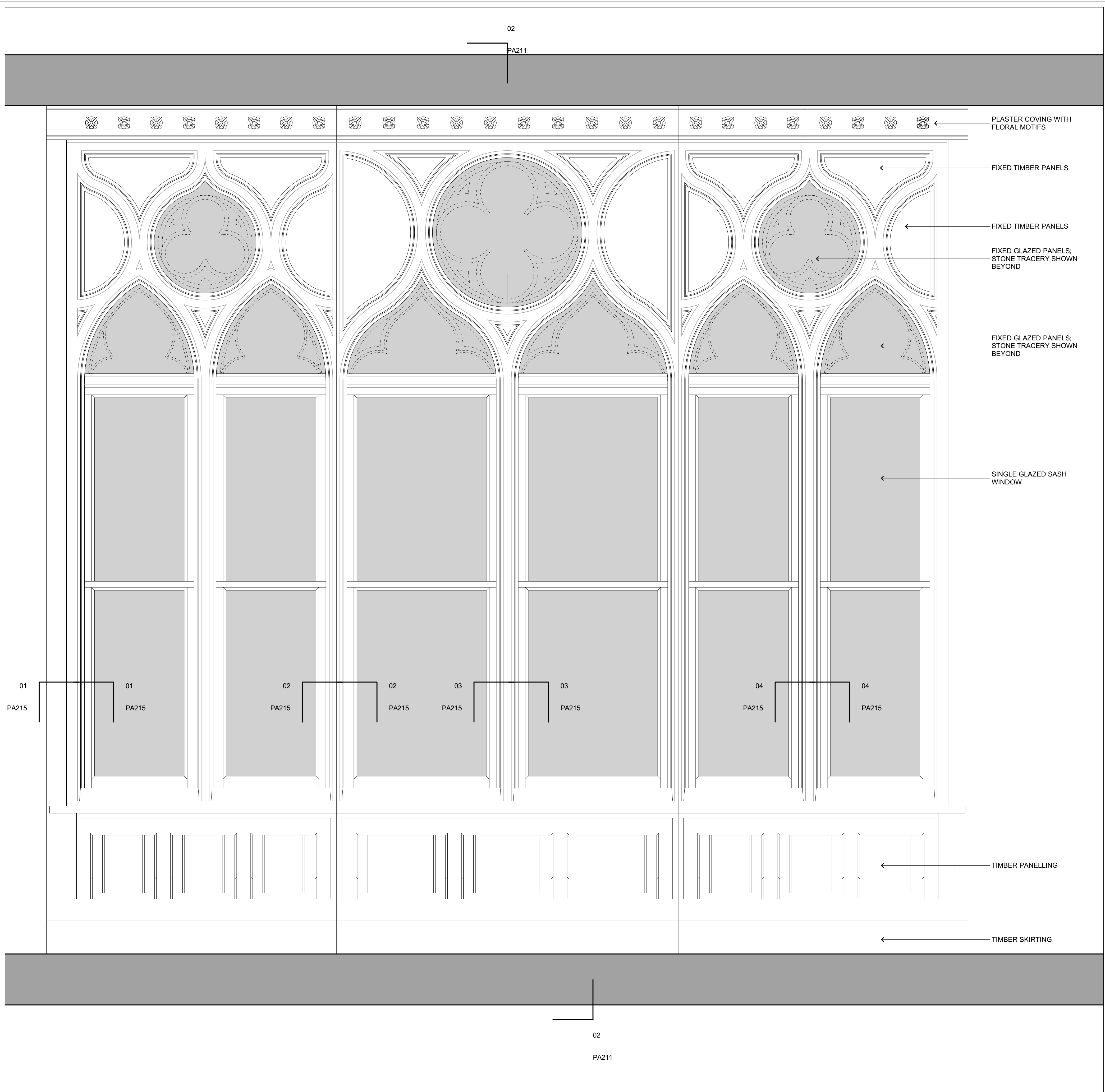
UNFOLDED INTERNAL ELEVATION OF EXISTING BAY WINDOW
