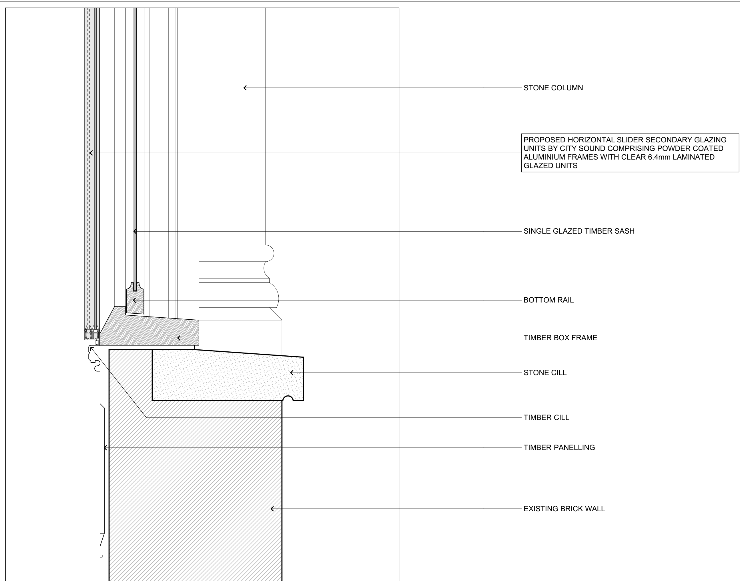
1 PROPOSED SECTIONAL DETAIL THROUGH CILL
