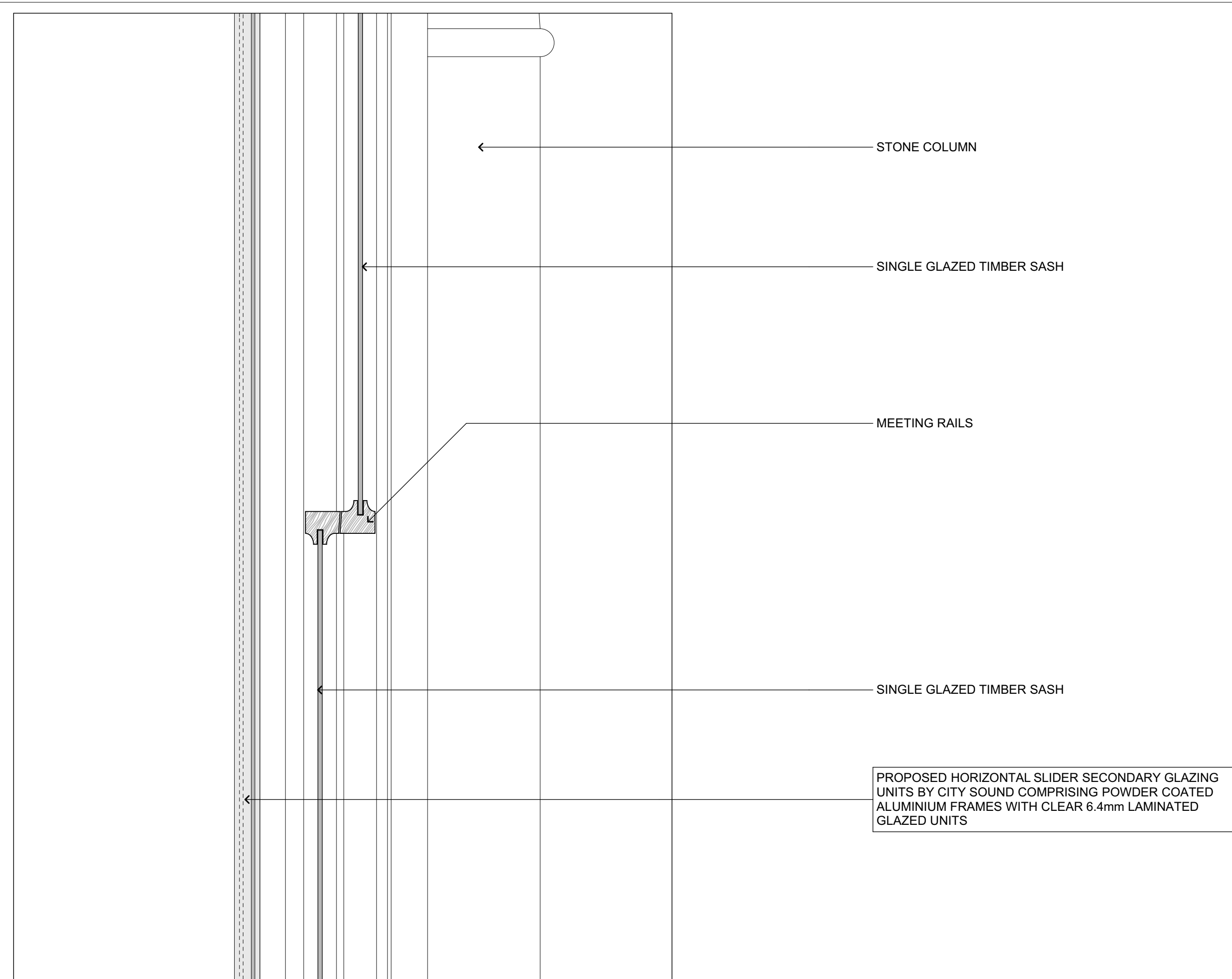
2 PROPOSED SECTIONAL DETAIL THROUGH MEETING RAIL
