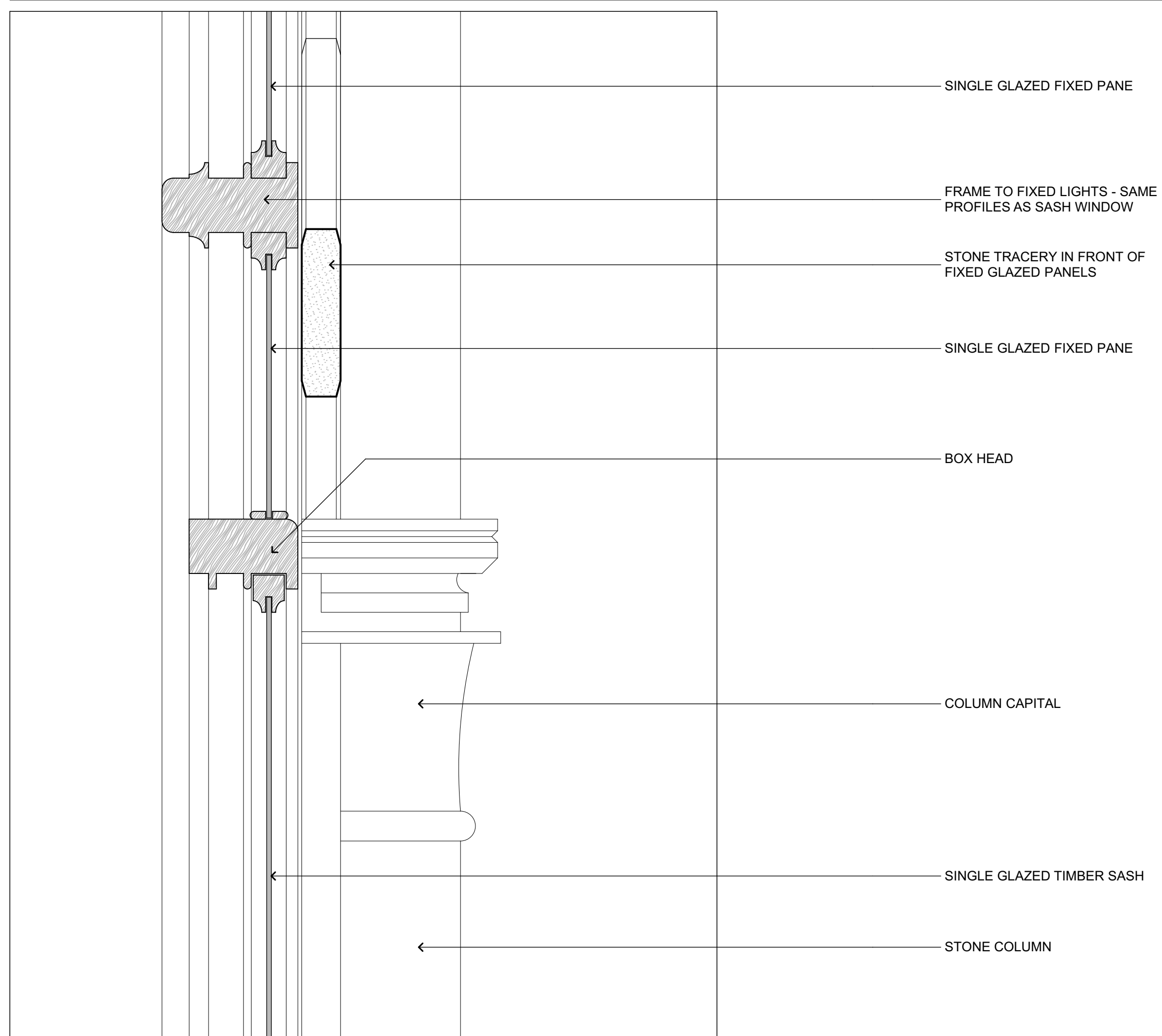
SECTIONAL DETAIL THROUGH HEAD OF SASH
