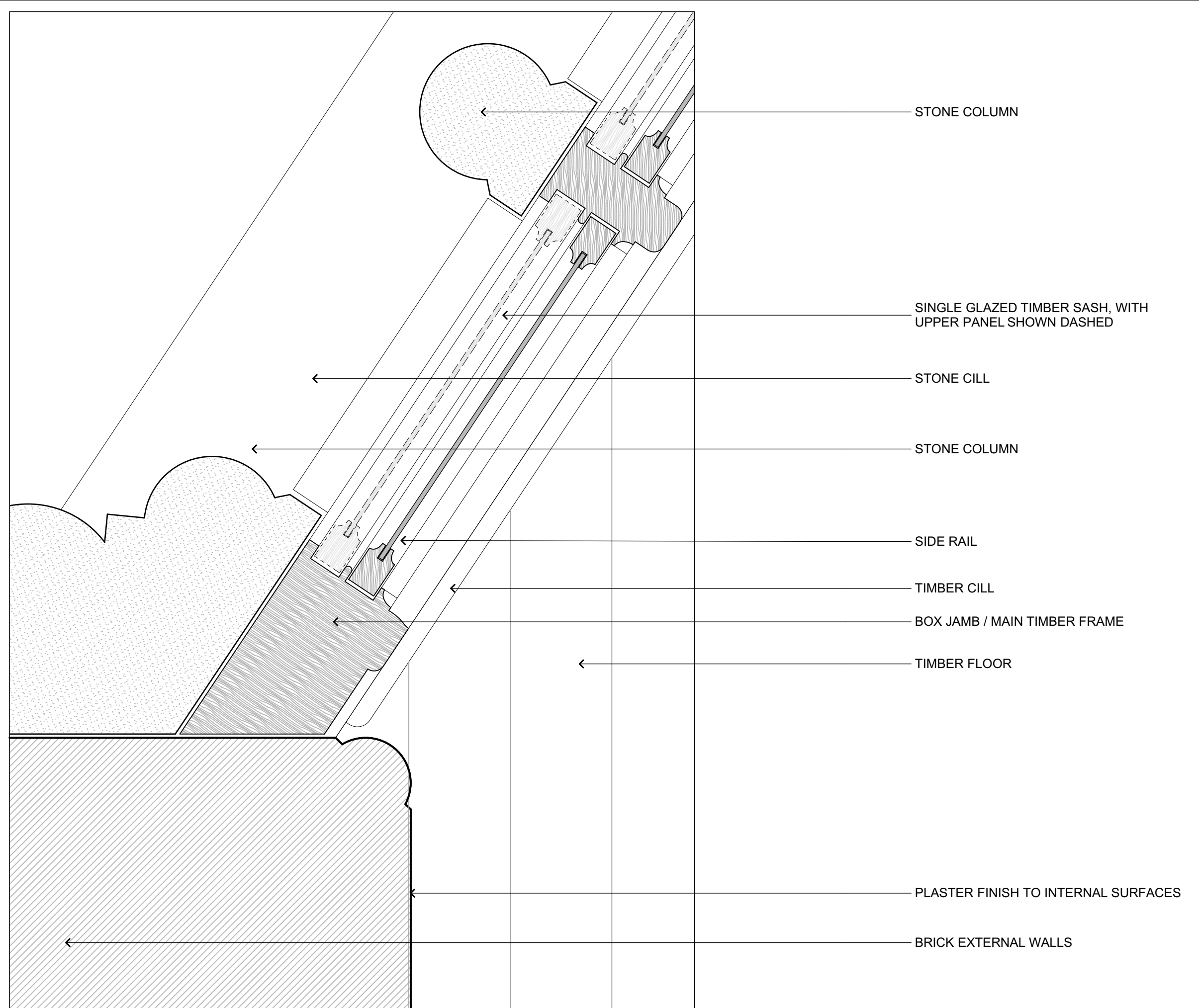
1 SIDE PANEL JAMB DETAIL
