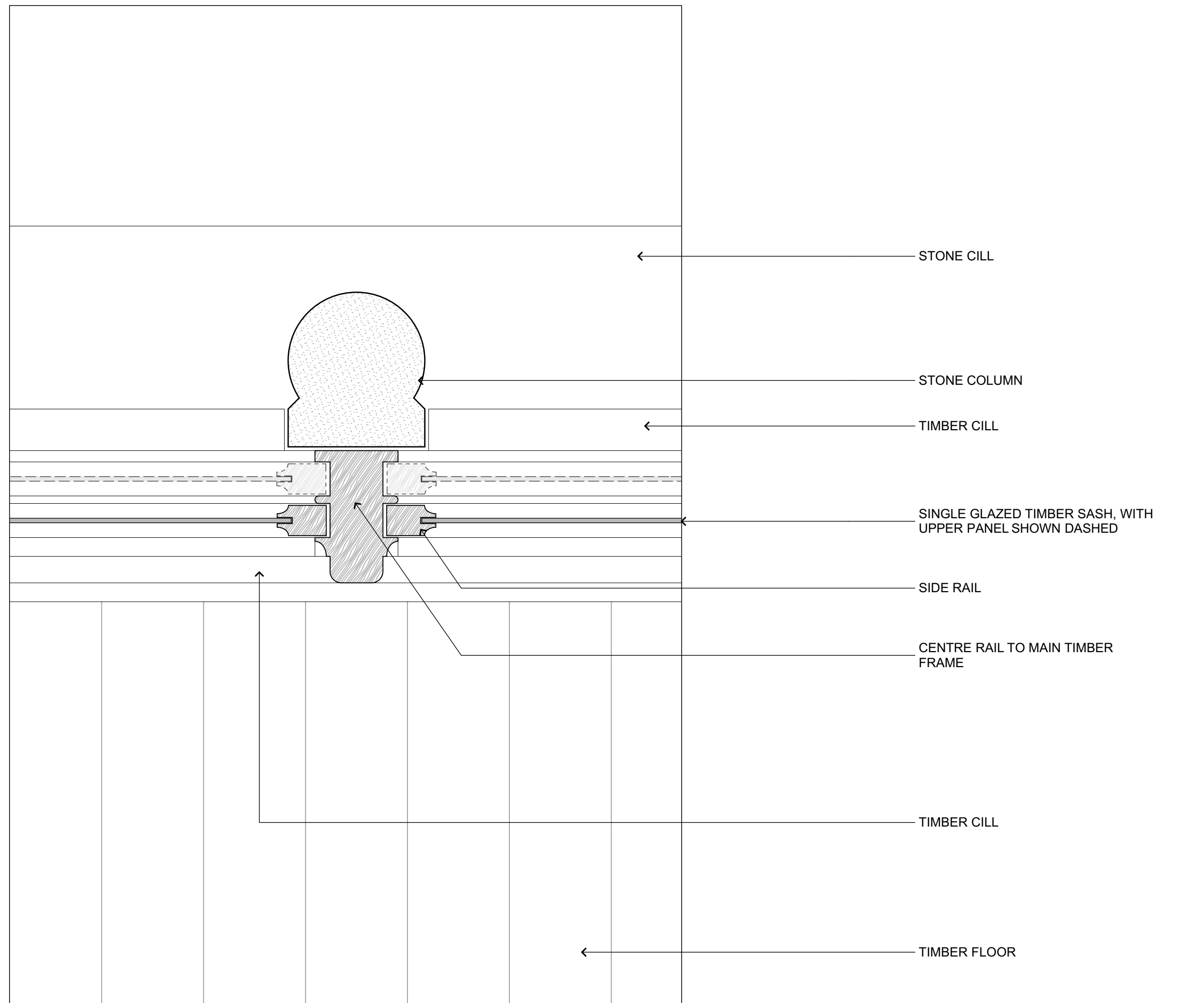
3 DETAIL OF JUNCTION BETWEEN STONE AND WINDOW CENTRE MULLION
