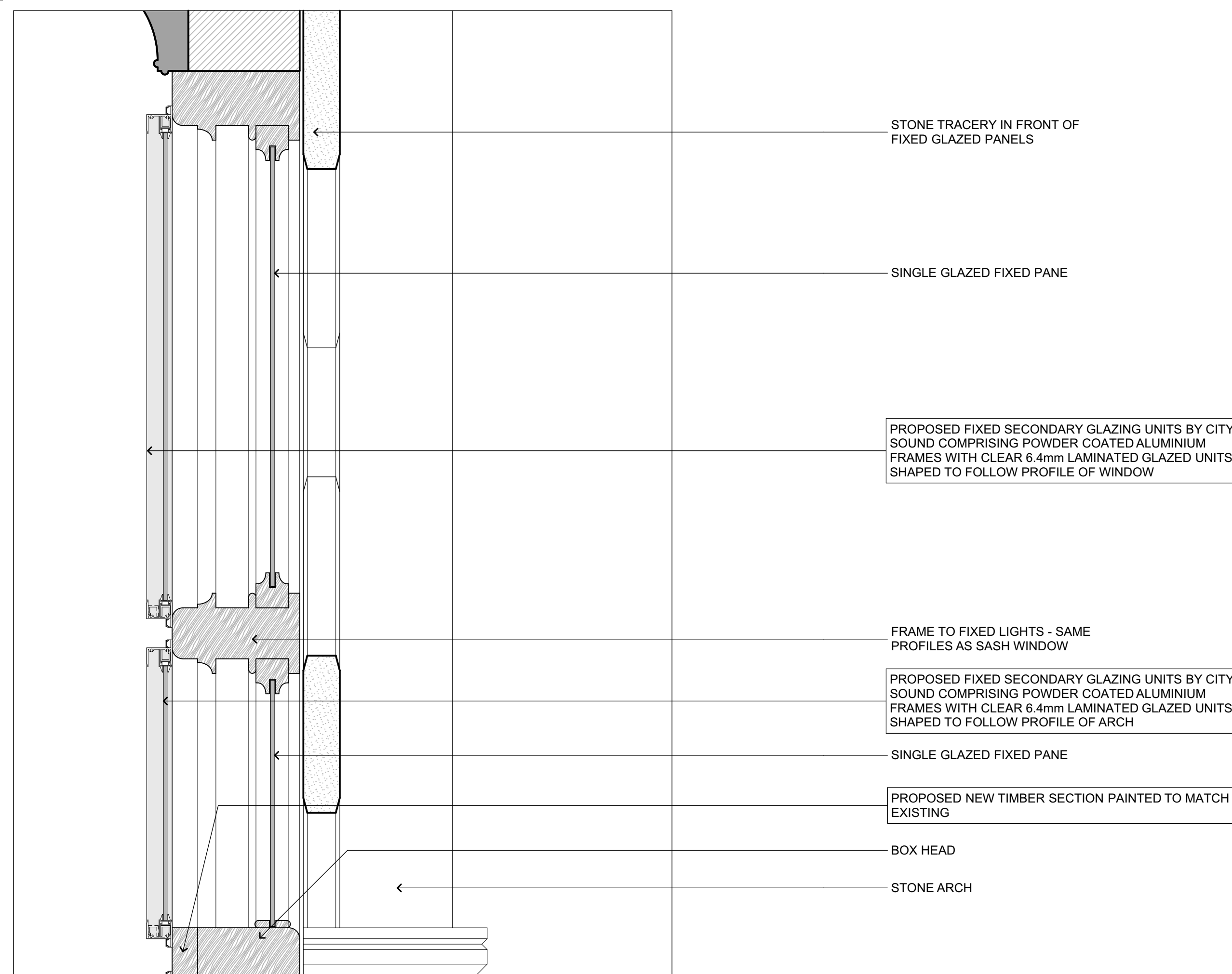
4 PROPOSED SECTIONAL DETAIL THROUGH FIXED LIGHTS ABOVE SASH WINDOW
