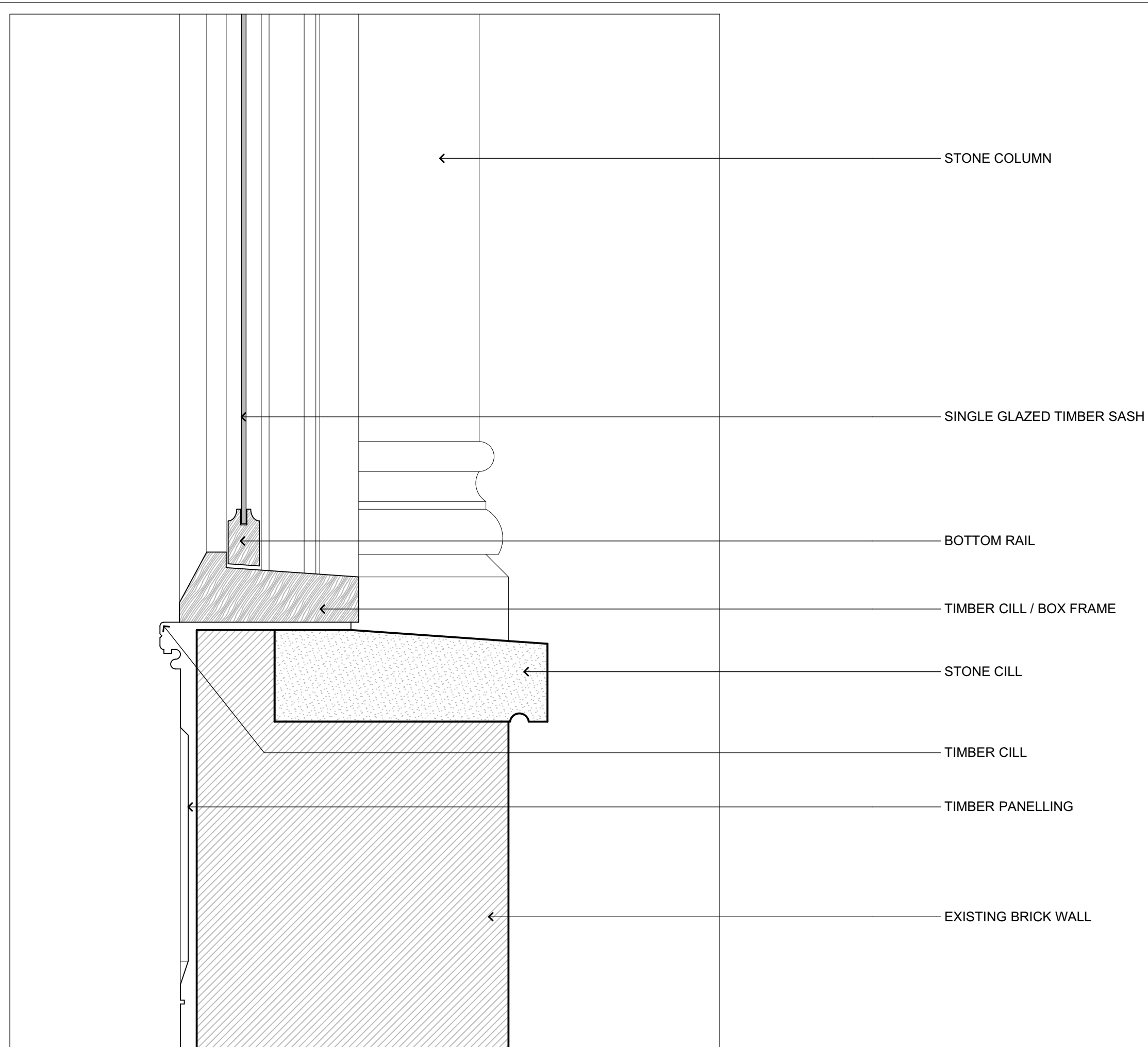
SECTIONAL DETAIL THROUGH CILL
