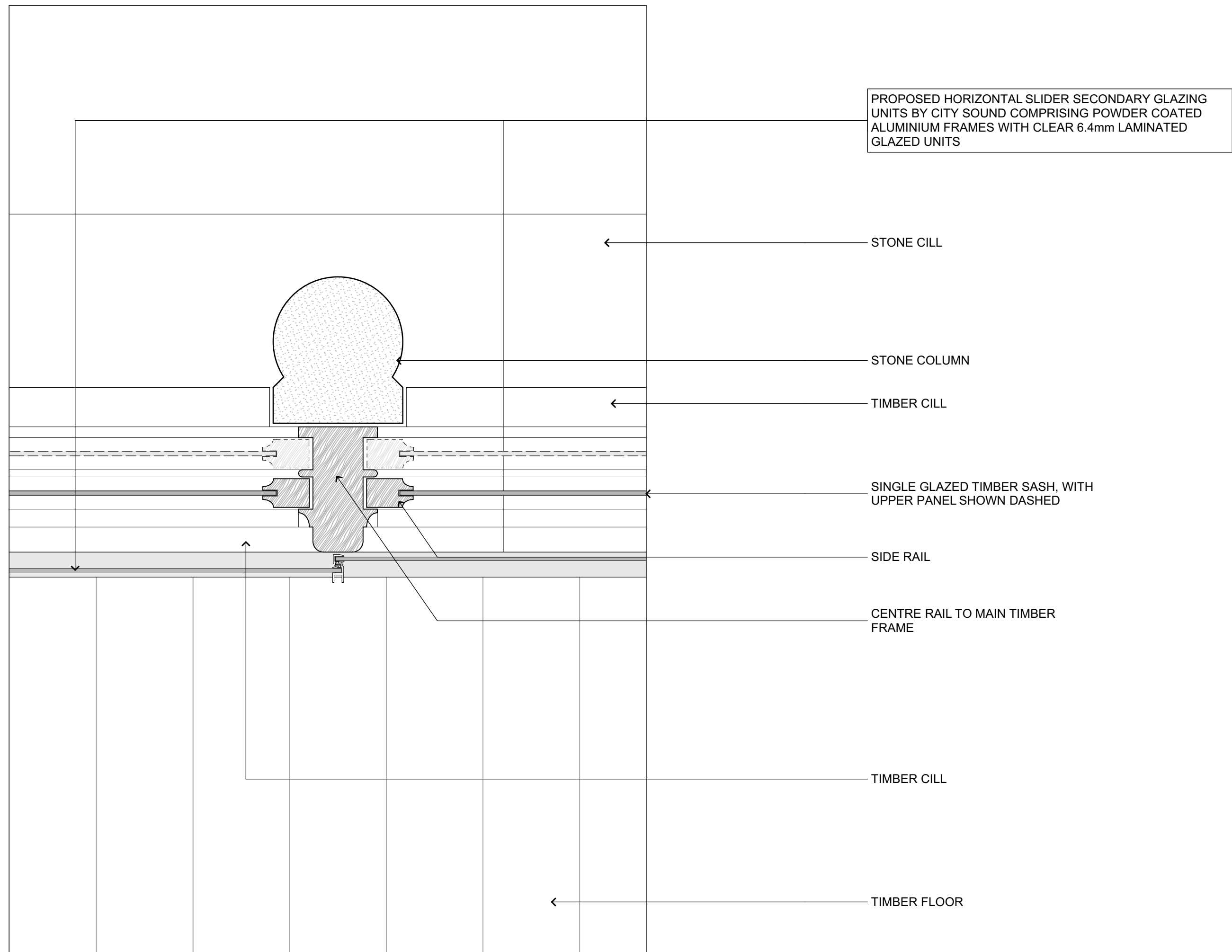
3 PROPOSED DETAIL OF JUNCTION BETWEEN STONE AND WINDOW CENTRE MULLION
