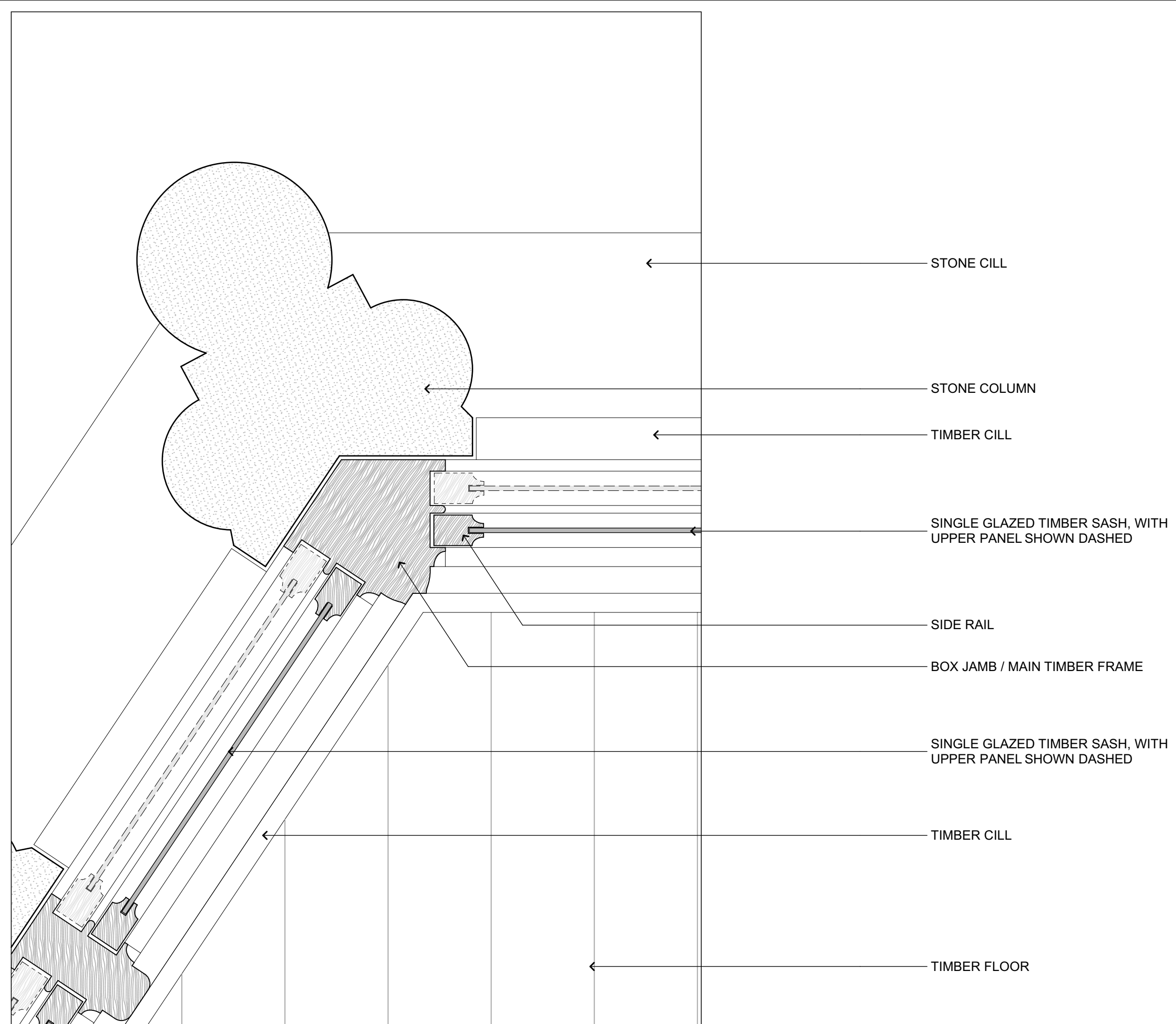
1:5 2 DETAIL OF JUNCTION BETWEEN TWO WINDOWS
