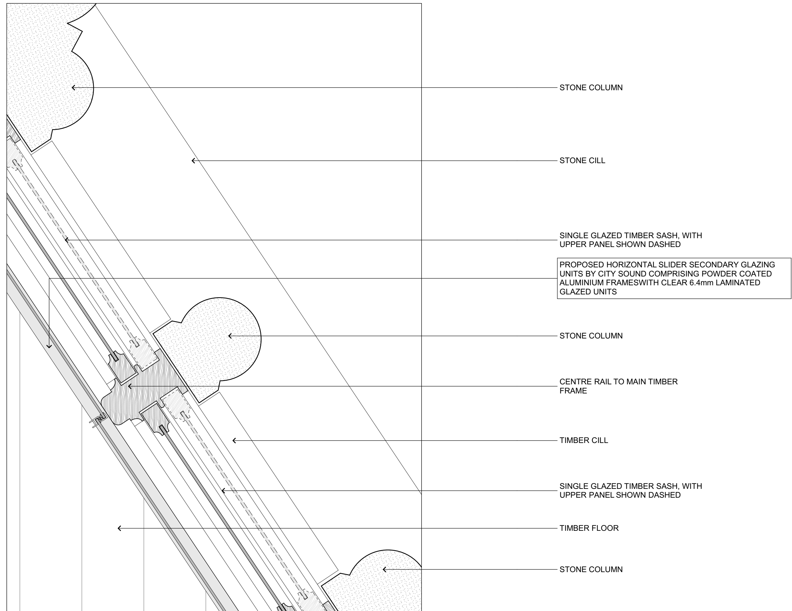
1:5 4 PROPOSED CENTRE MULLION DETAIL TO SIDE WINDOWS
