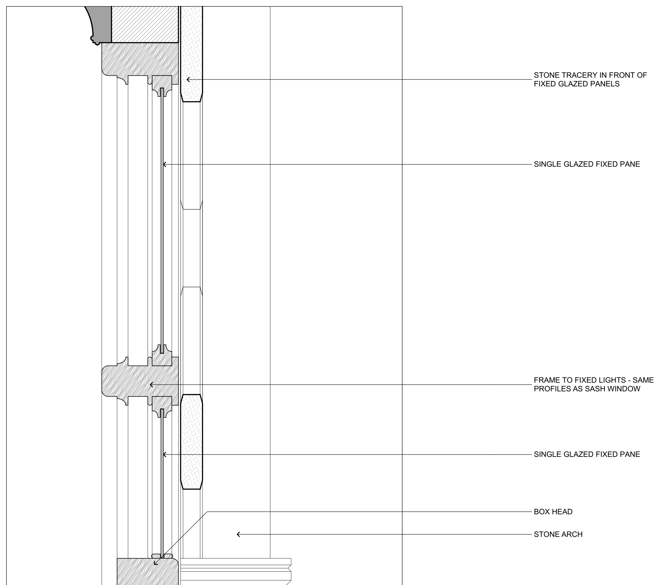
SECTIONAL DETAIL THROUGH FIXED LIGHTS ABOVE SASH WINDOW
