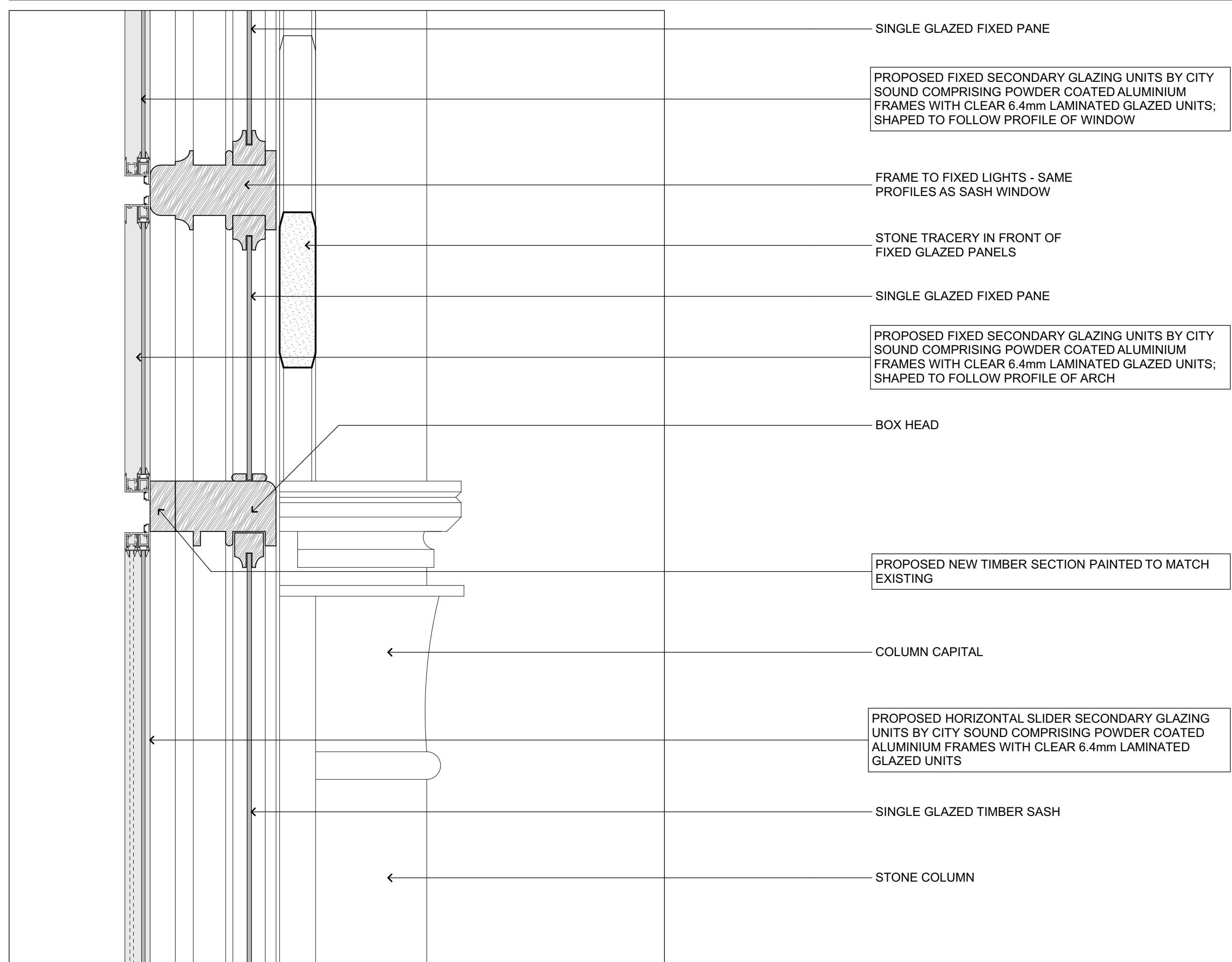
3 PROPOSED SECTIONAL DETAIL THROUGH HEAD OF SASH
