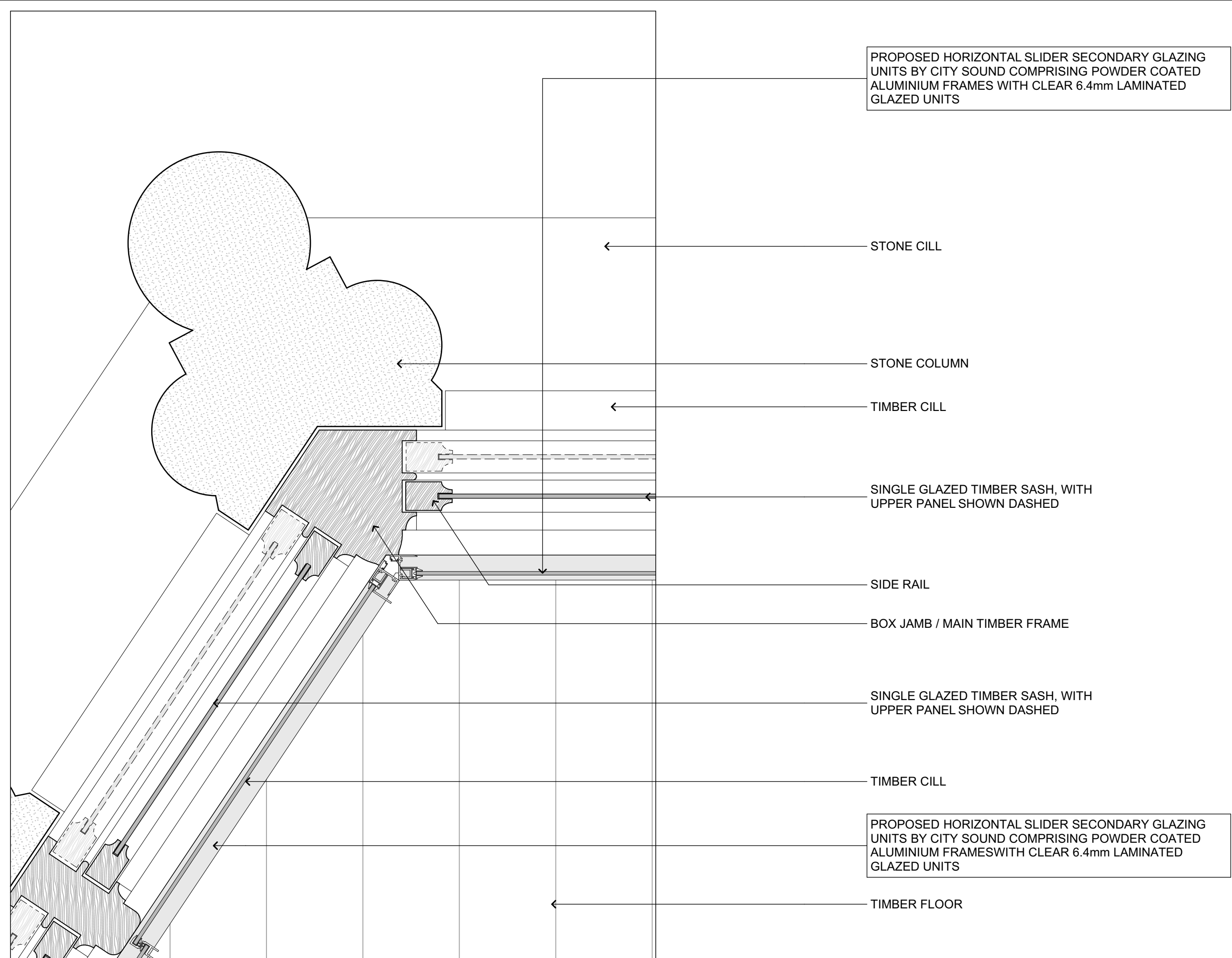
1:5 2 PROPOSED DETAIL OF JUNCTION BETWEEN TWO WINDOWS
