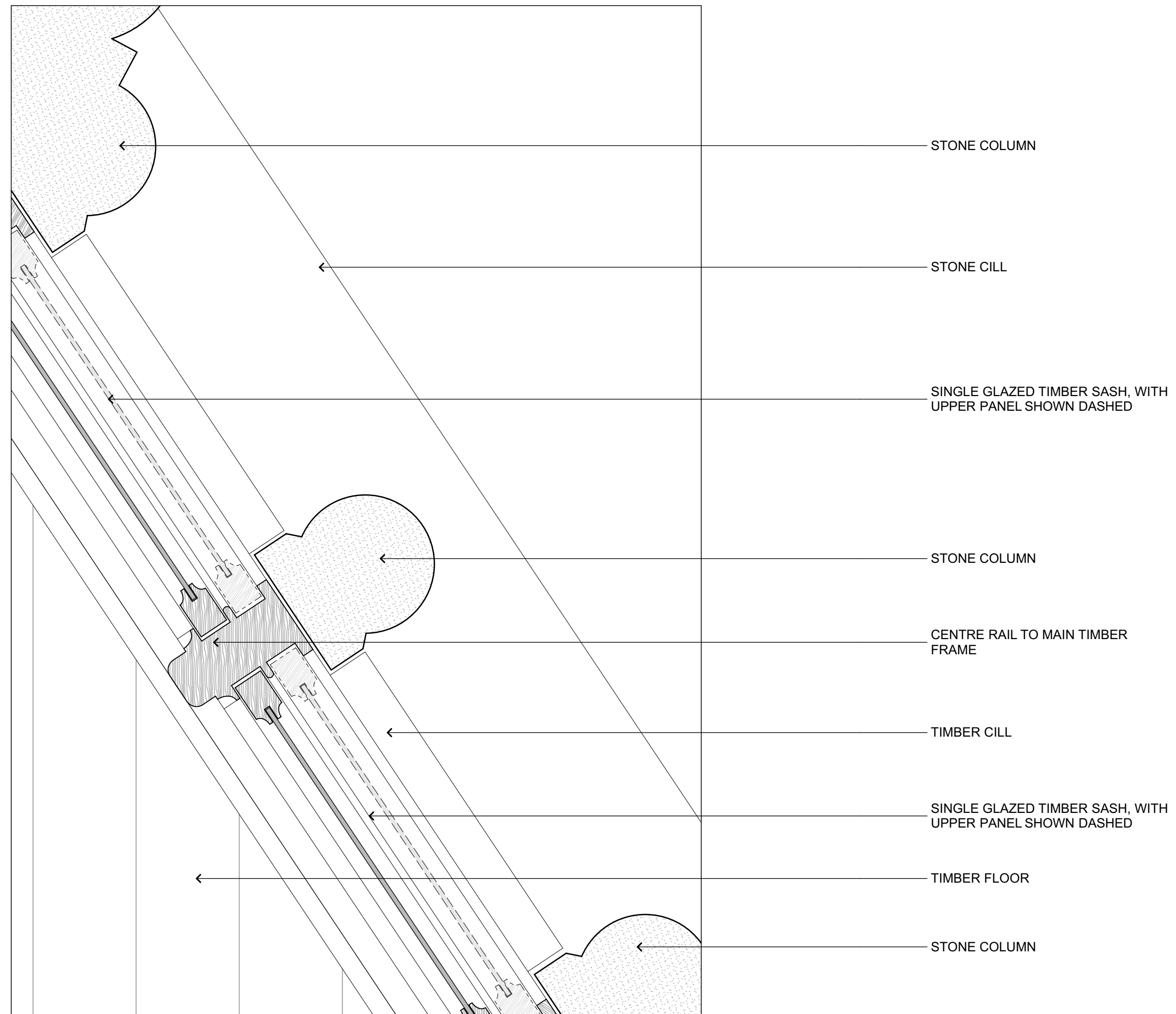
1:5 4 CENTRE MULLION DETAIL TO SIDE WINDOWS
