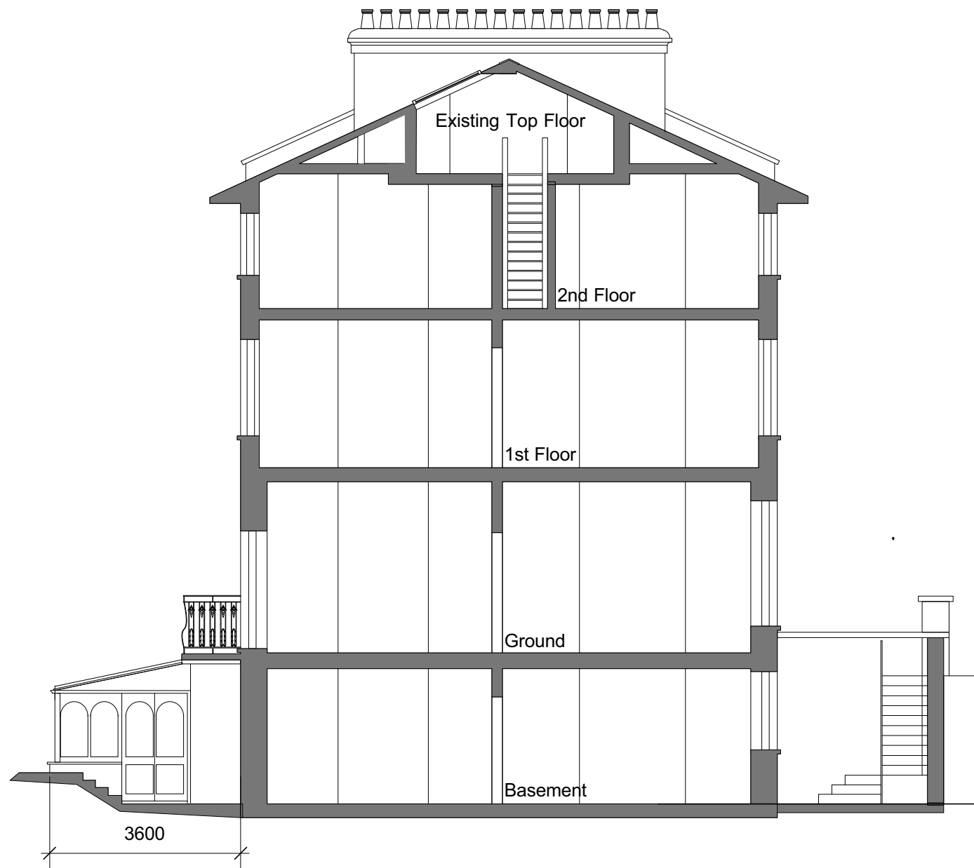
Section AA
