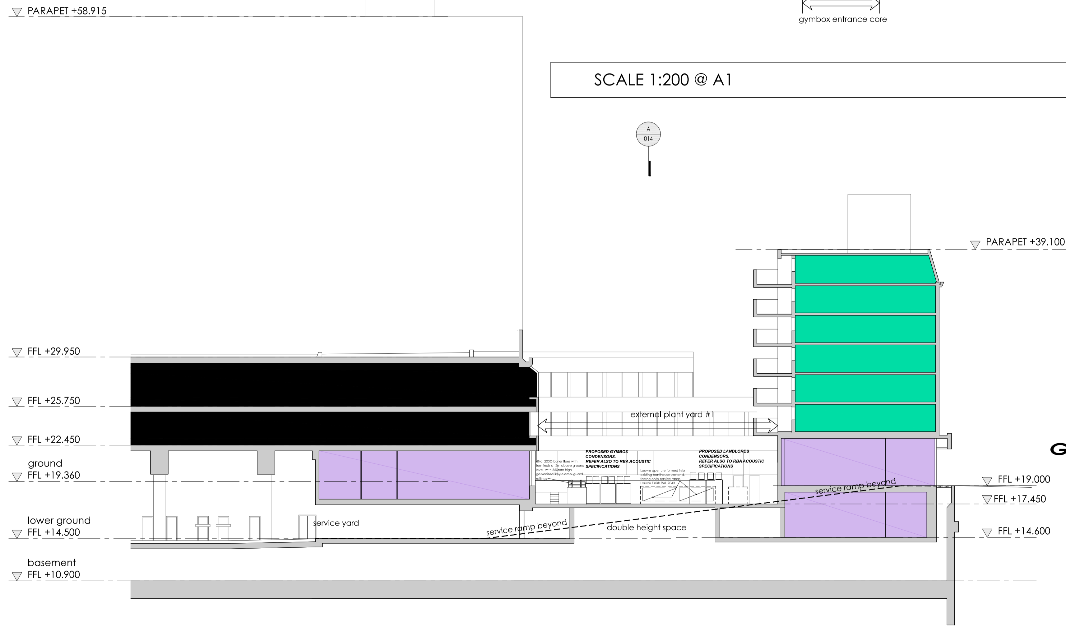
SCALE 1:200 @ A1
