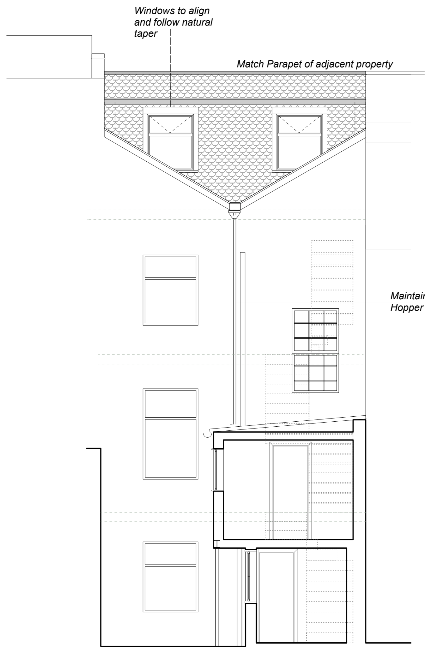
Rear Elevation
