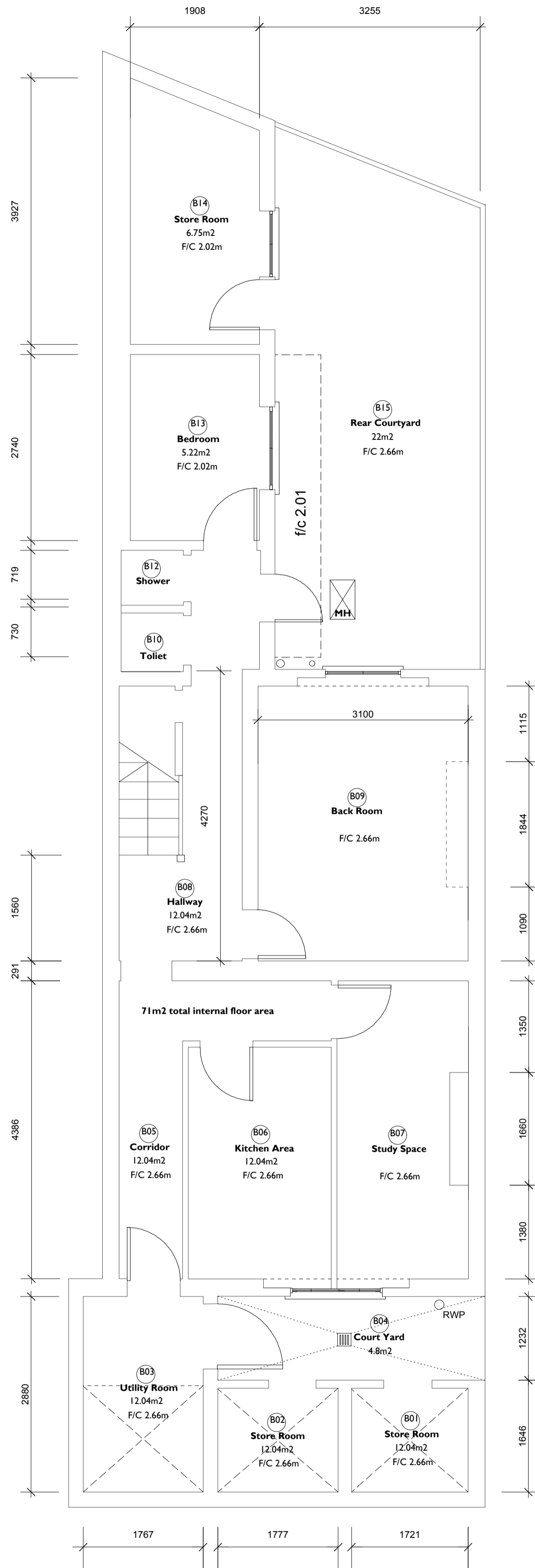
Basement Plan
