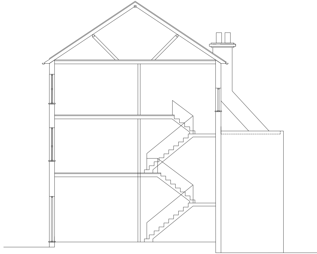
SECTION AS EXISTING
