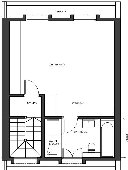
05- ROOF PLAN
