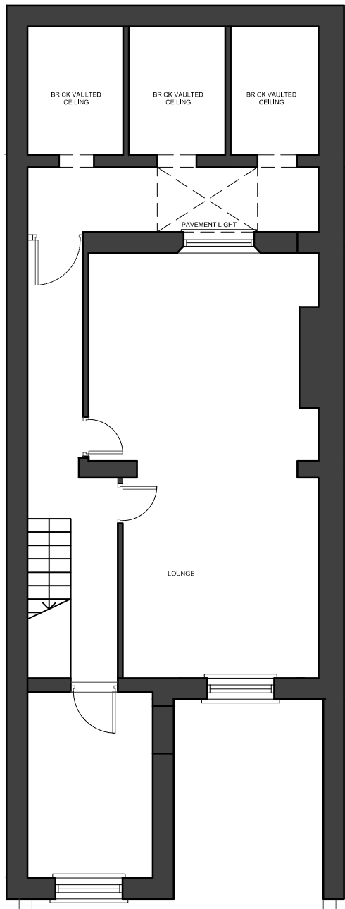
01- LOWER GROUND FLOOR PLAN
