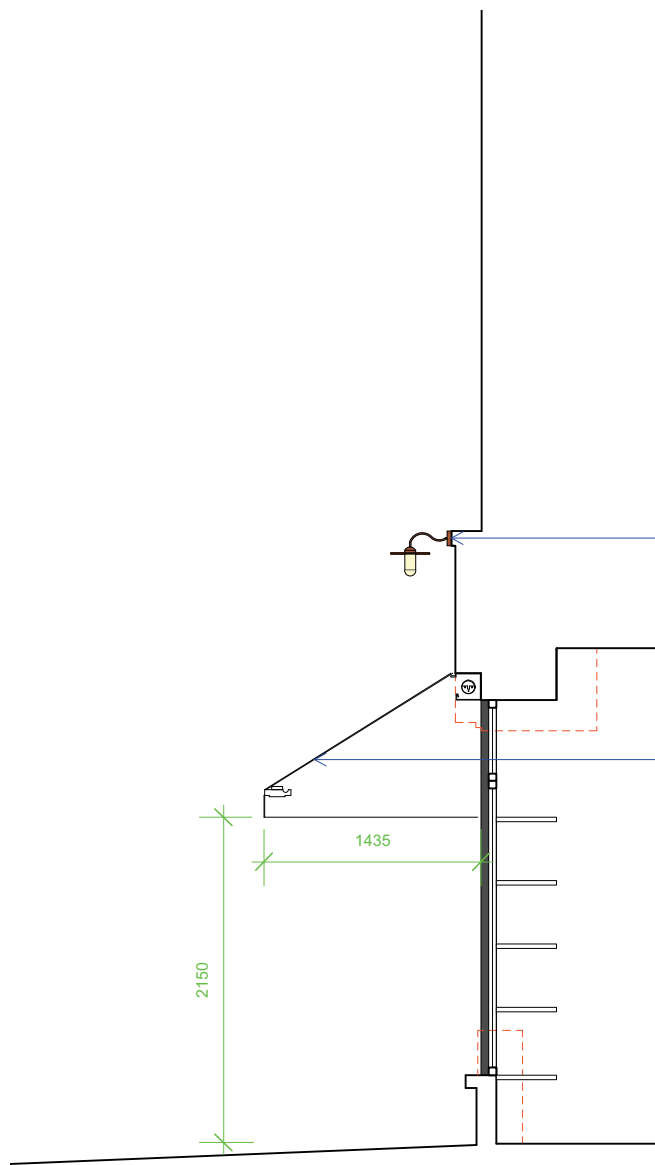
PROPOSED SECTION 00
