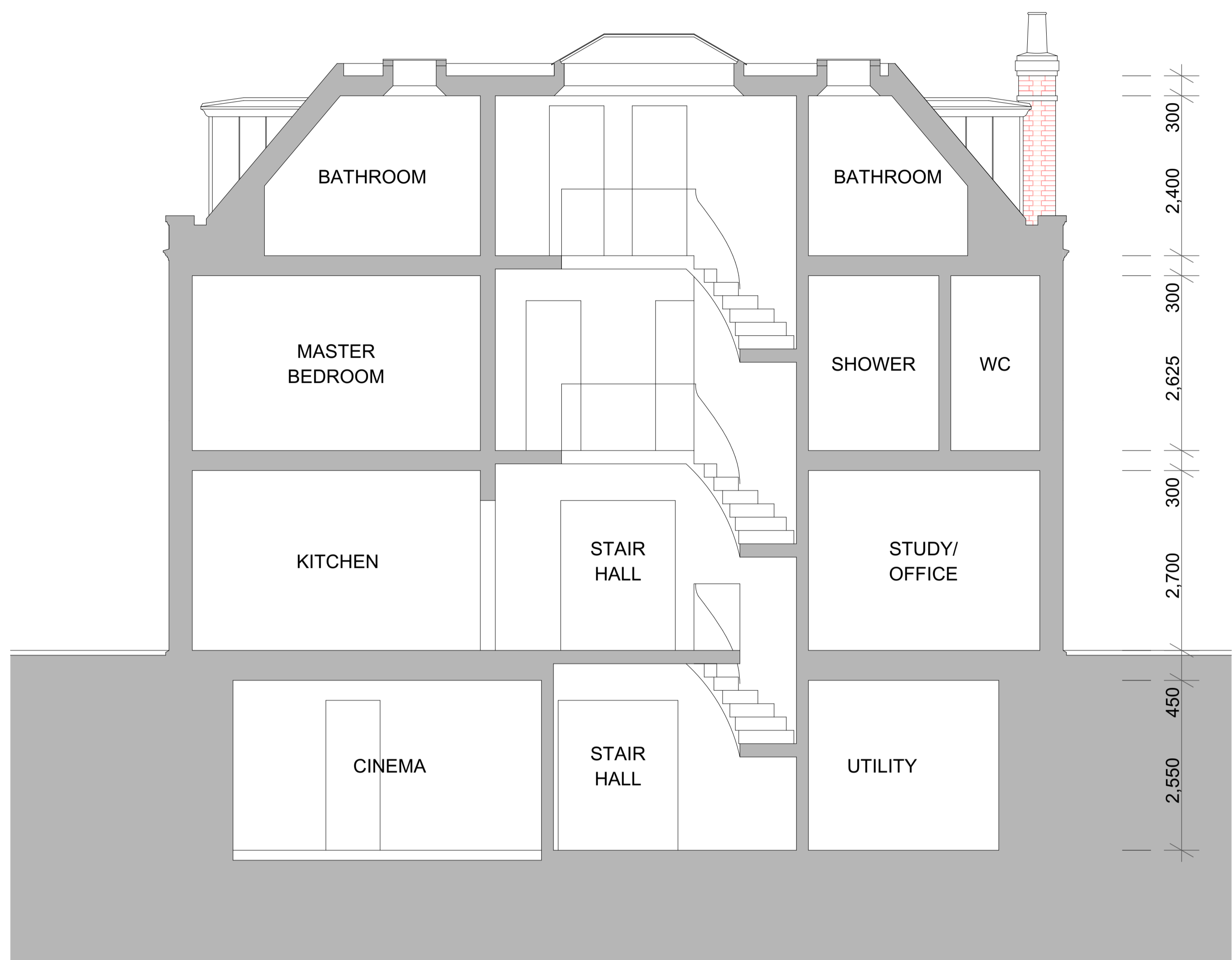
CROSS SECTION
