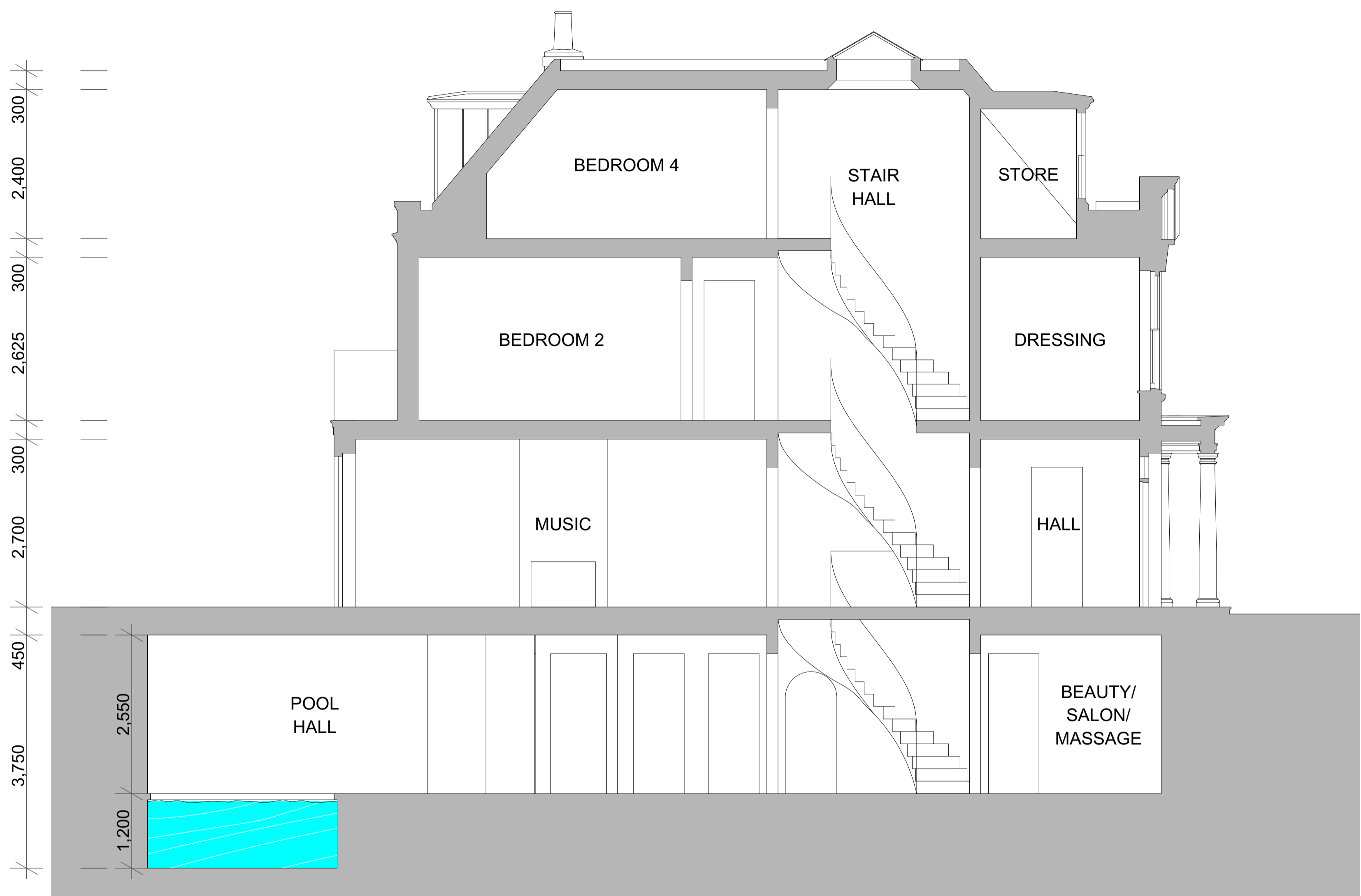
LONG SECTION
