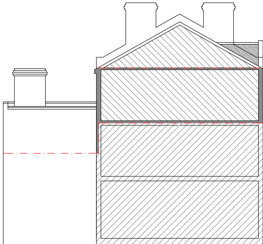
Side Elevation
