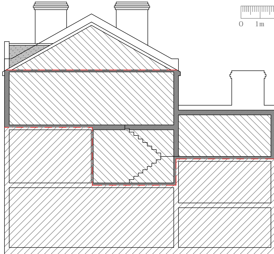
Side Elevation
