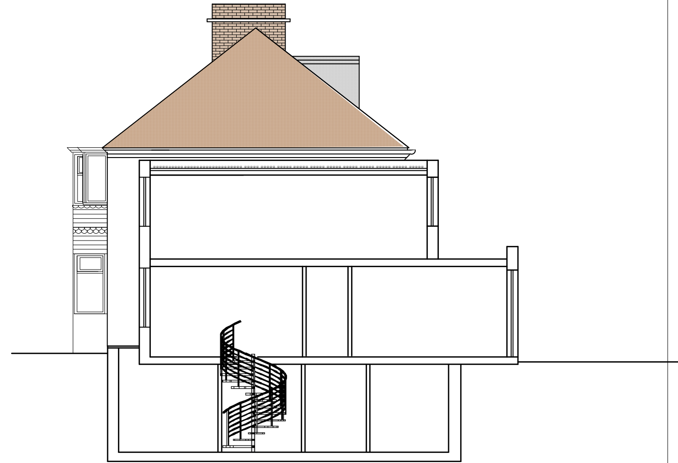
Cross Section BB
