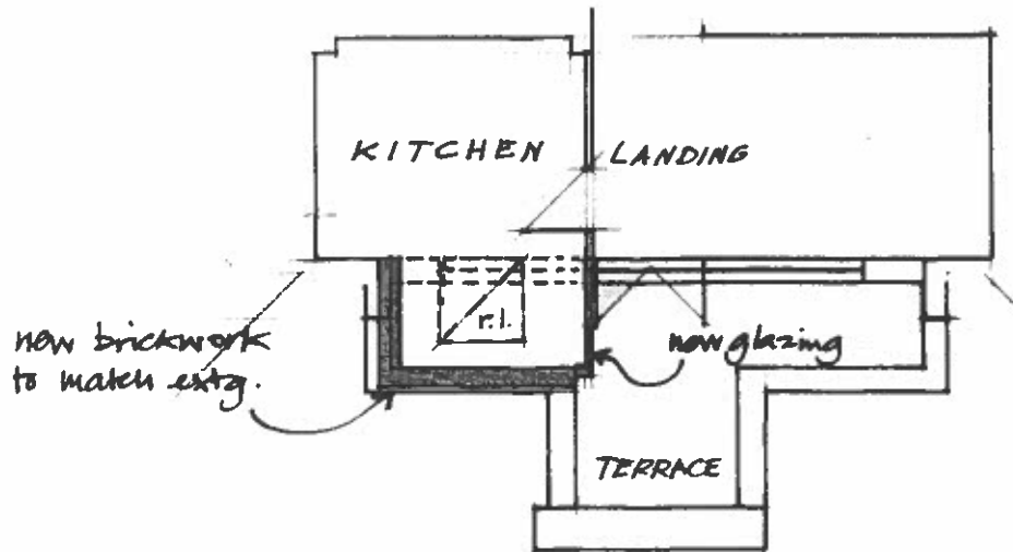
PROPOSED PLAN 1:100
