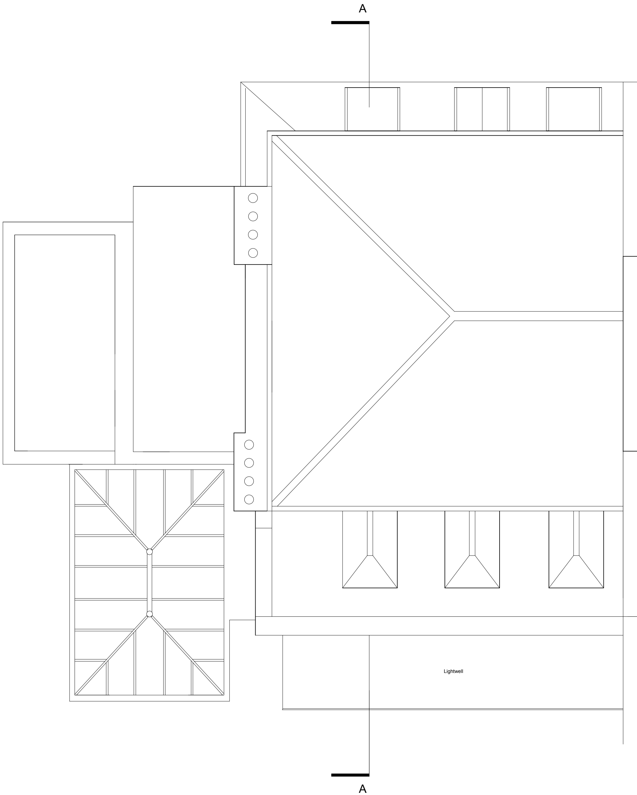
EXISTING ROOF PLAN SHOWING LIGHTWELL
