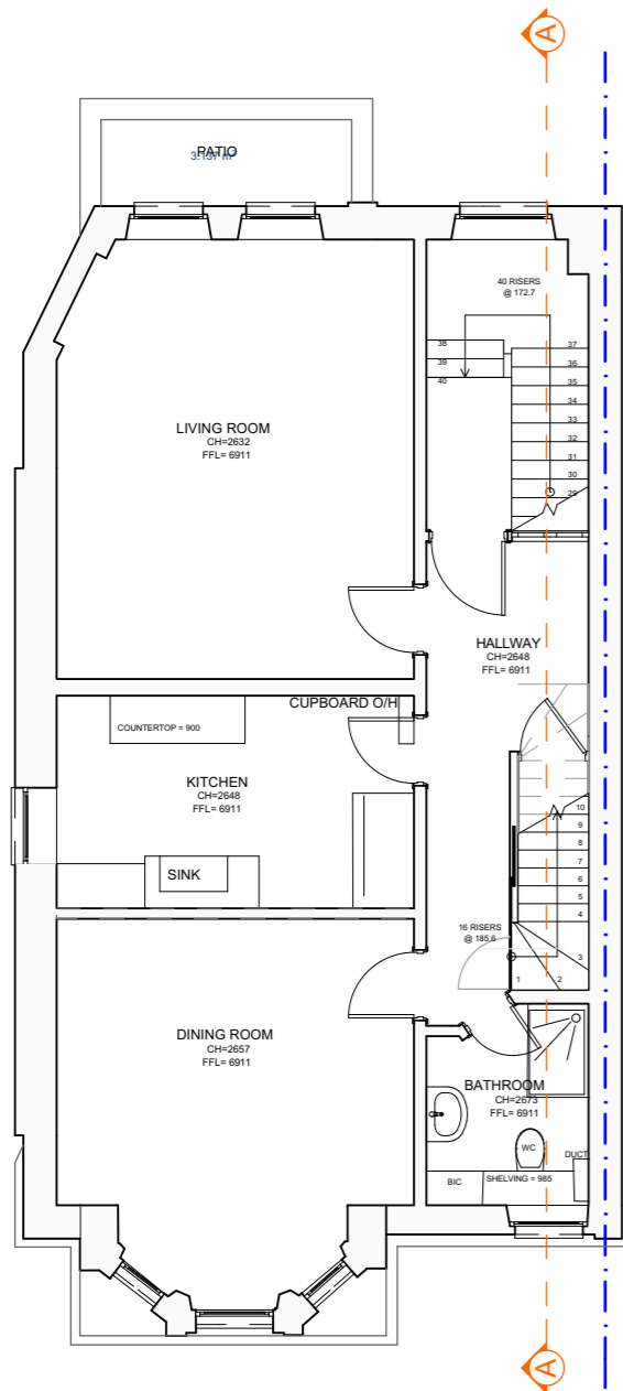
Second Floor Plan 1:100
