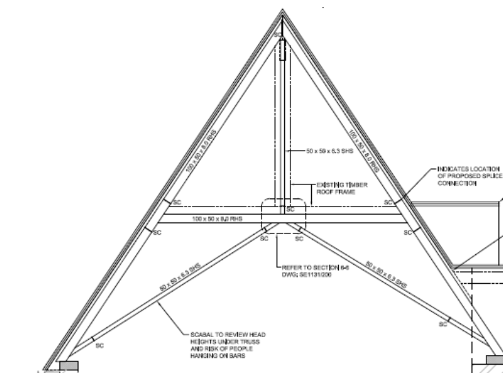
Fig 4 – Detail of proposed new roof truss
