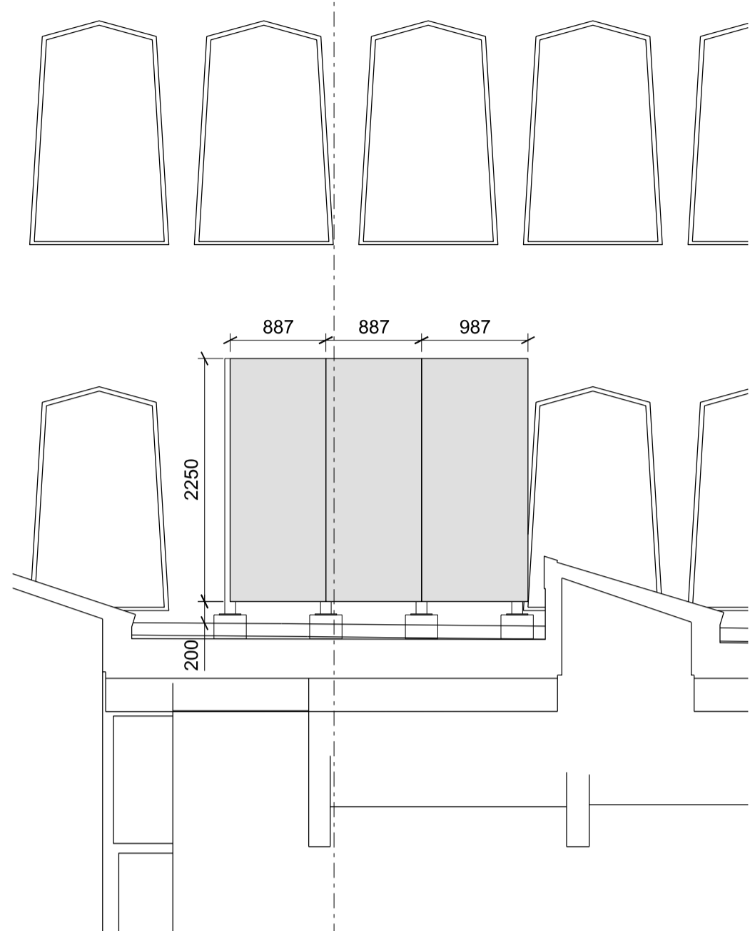
01 LOUVRE DETAIL Scale 1:50
