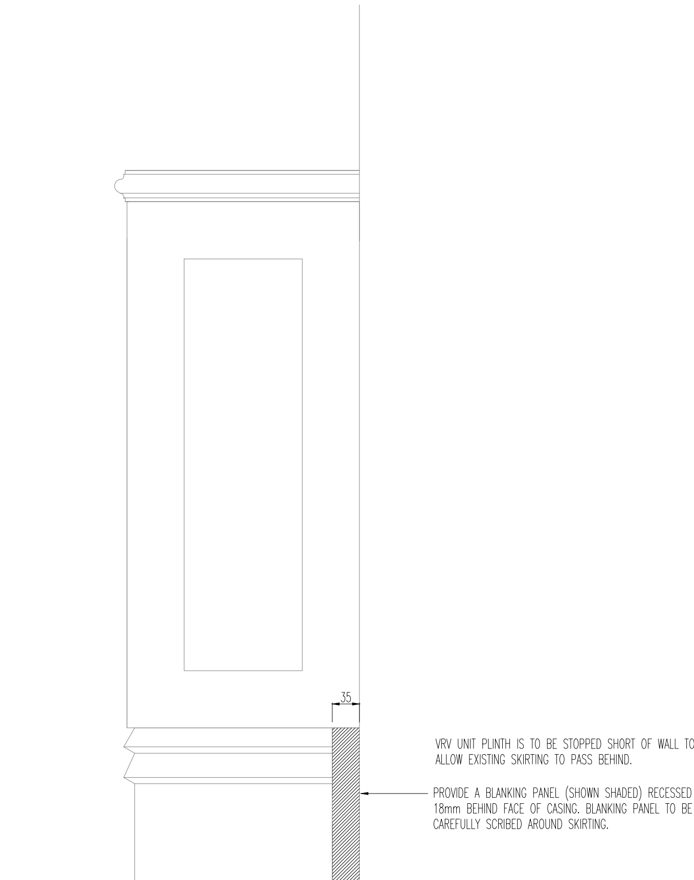
SIDE VIEW
