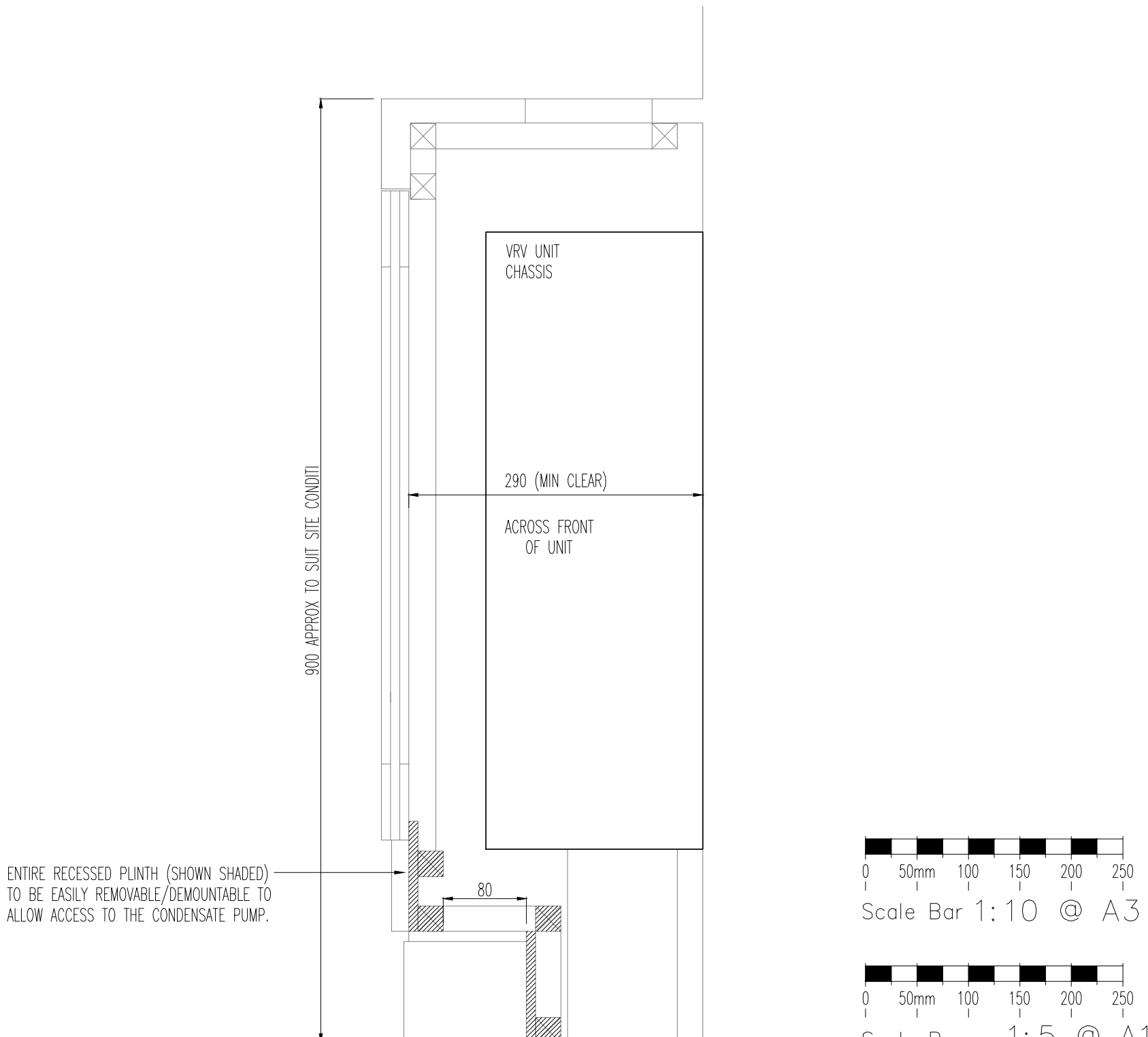
SECTION
