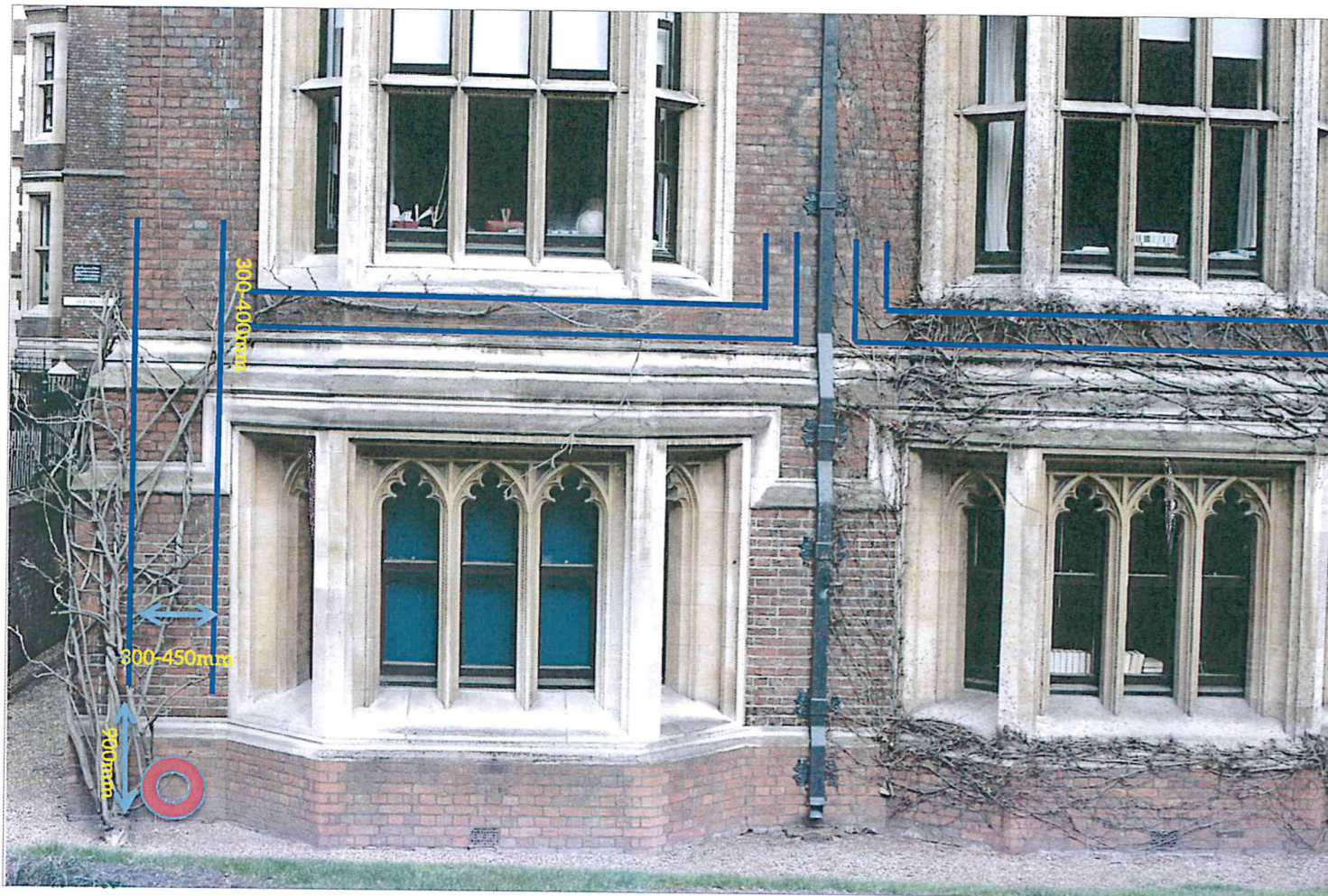
(North) East elevation
