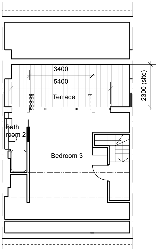
SECOND FLOOR
