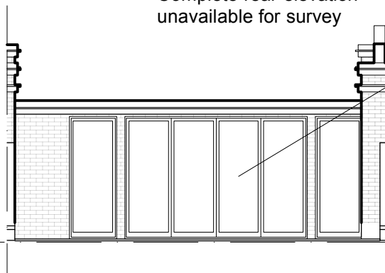
REAR ELEVATION TO ROOF
