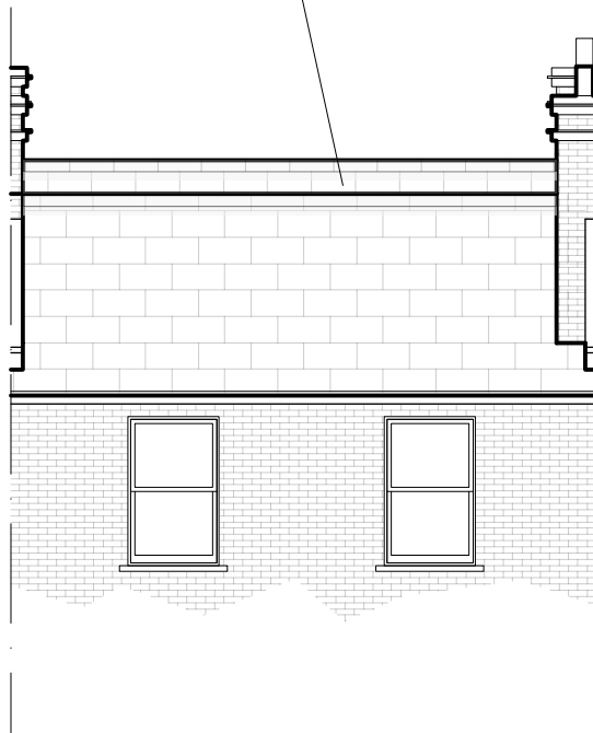
REAR ELEVATION
