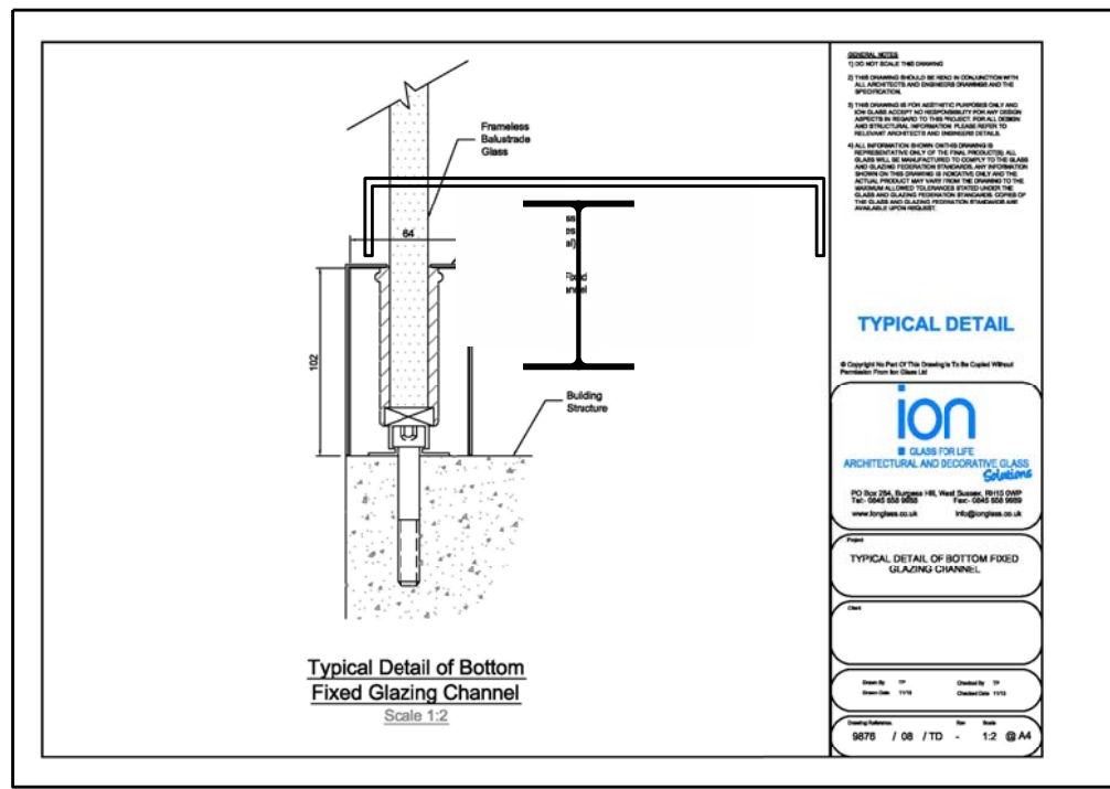
Typical stainless steel fixing detail to glass balustrade
