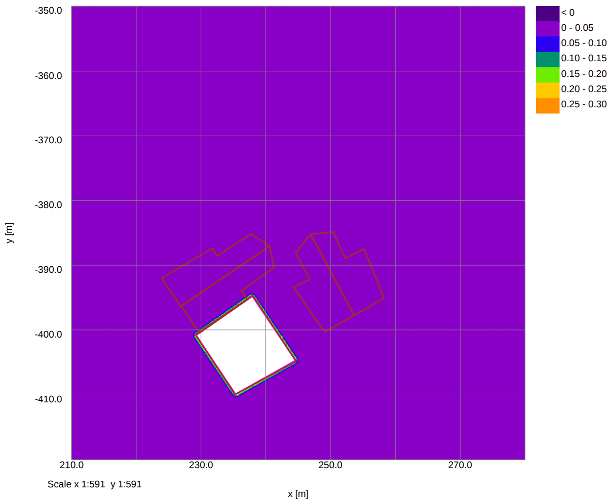
Vertical Settlement Contours: Grid 2 (level -2.150m) (Interval 0.05mm)
