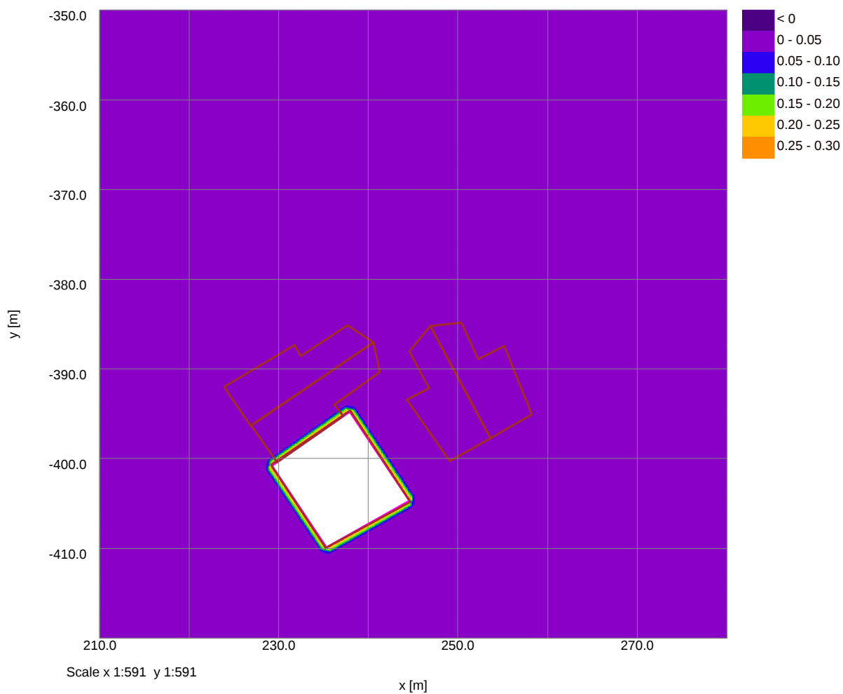
Horizontal Displacement Contours: Grid 2 (level -2.150m) Interval 0.05mm
