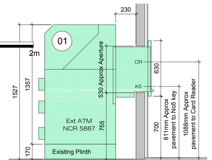
ATM No1 - Existing Section (scale 1:25 @ A3)
