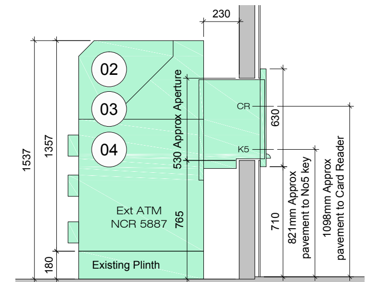
ATMs No2,3,4 - Existing Section (scale 1:25 @ A3)
