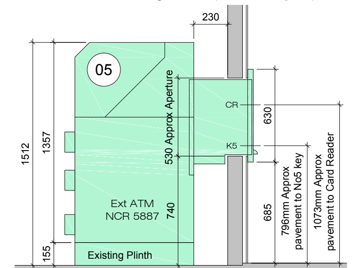
ATM No5 - Existing Section (scale 1:25 @ A3)
