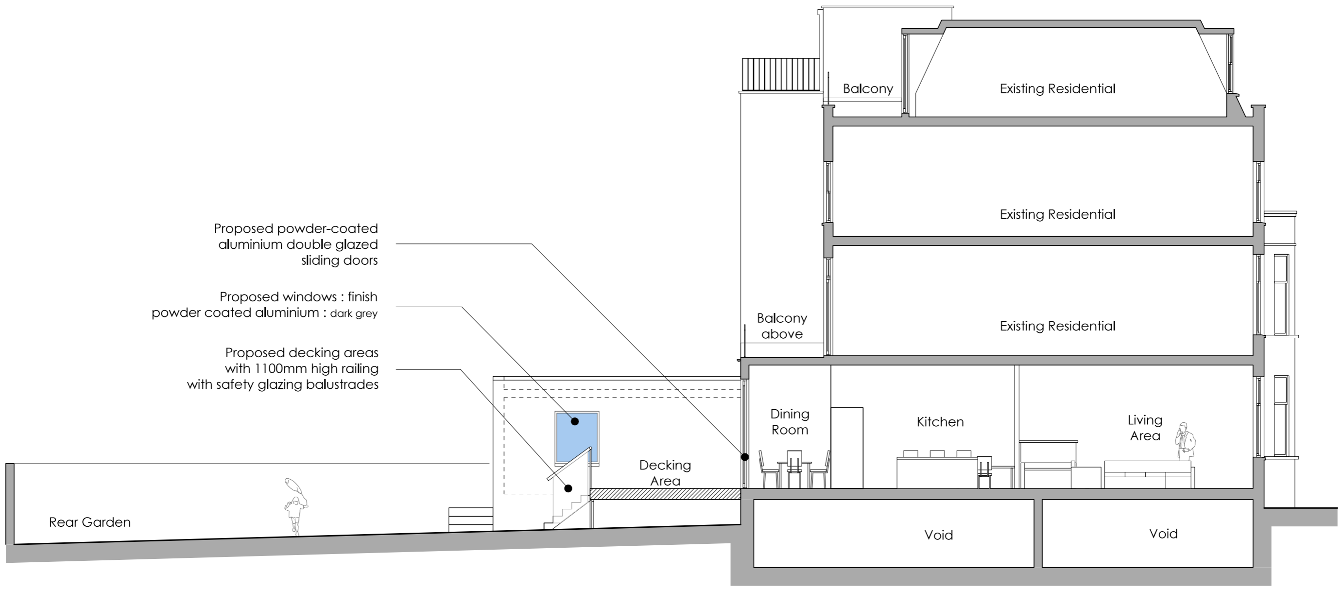
1 P-121 Proposed Side Elevation & Longitudinal Section scale 1:100 @ A3
