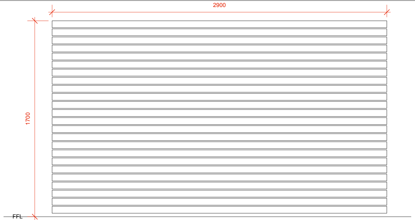
Privacy Screen: Western Red Cedar timber cladding H1.7m . Scale NTS.
