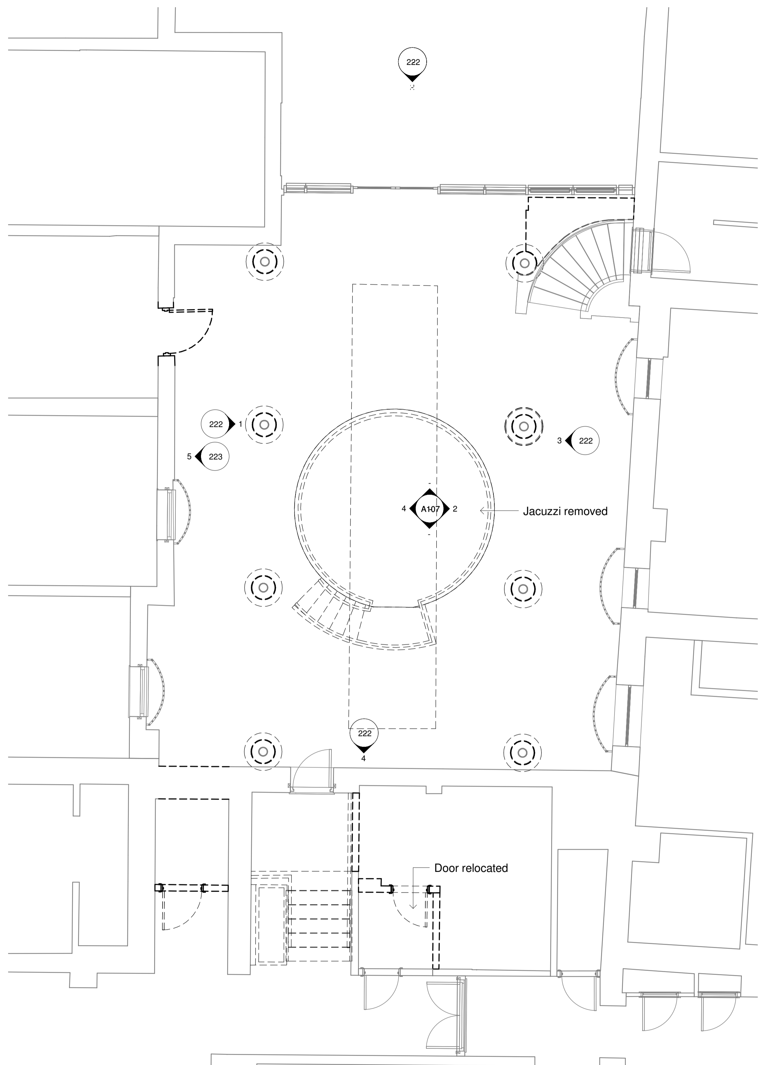
1 Demolition Ground Floor 1 : 50
