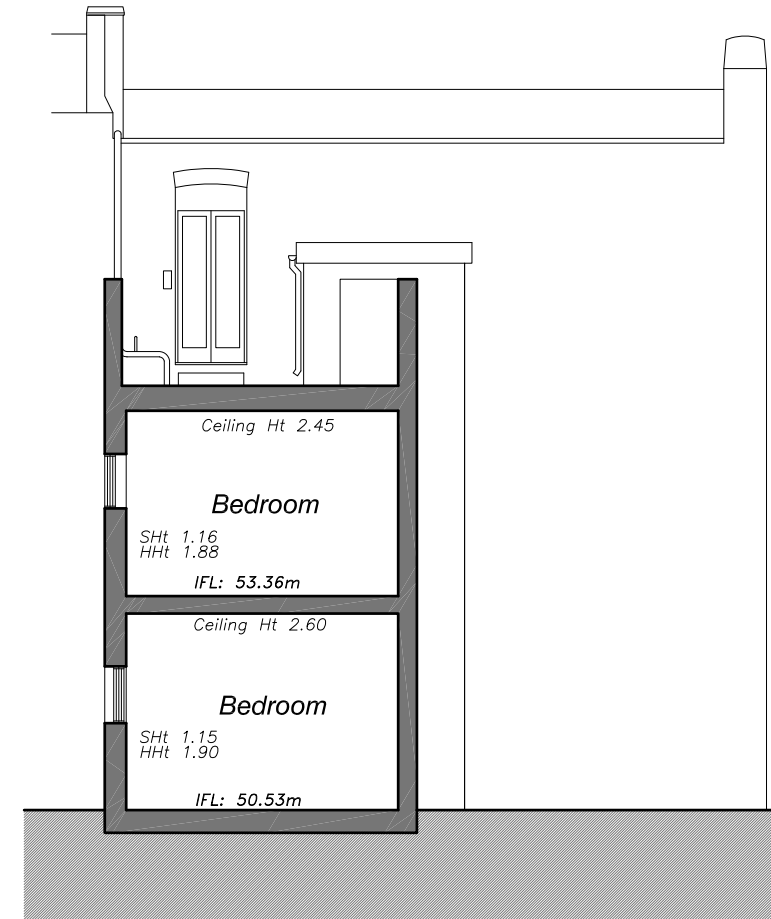
02 Section B
