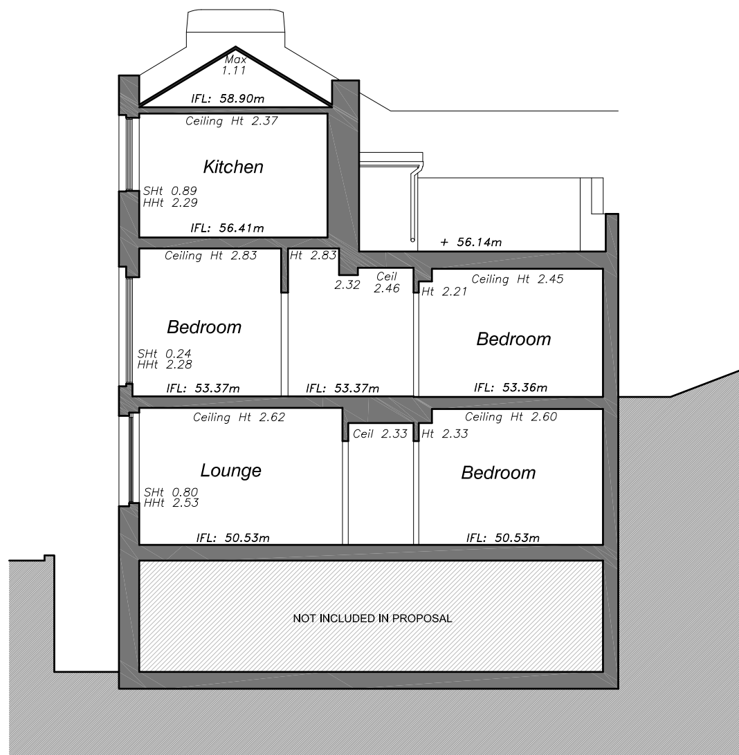
01 Section A
