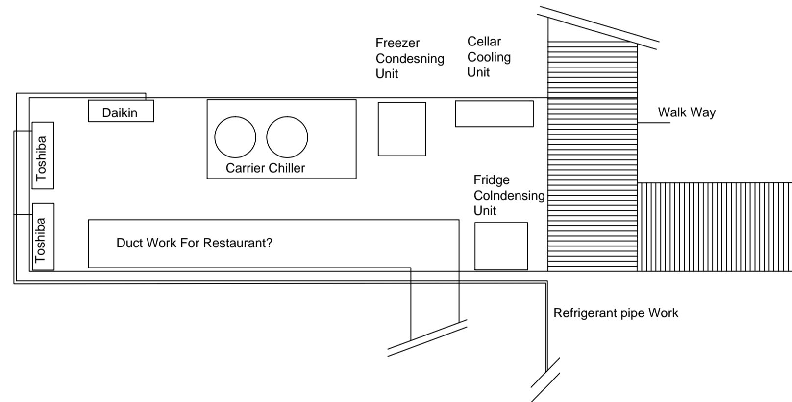
EXISTING ROOF PLANT LAYOUT
