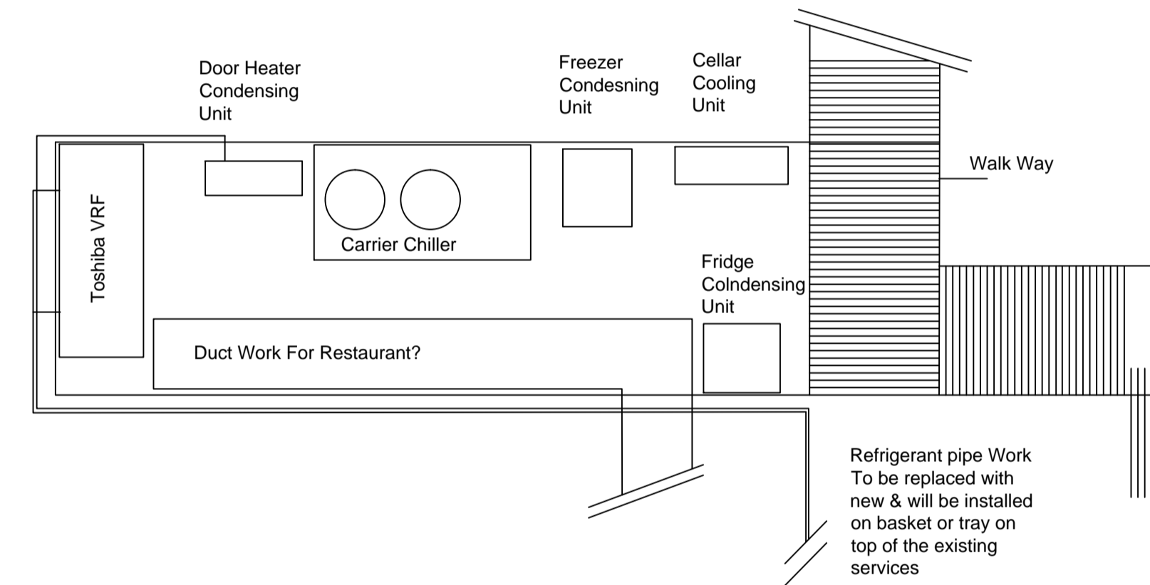
PROPOSED ROOF PLANT LAYOUT OPTION 1
