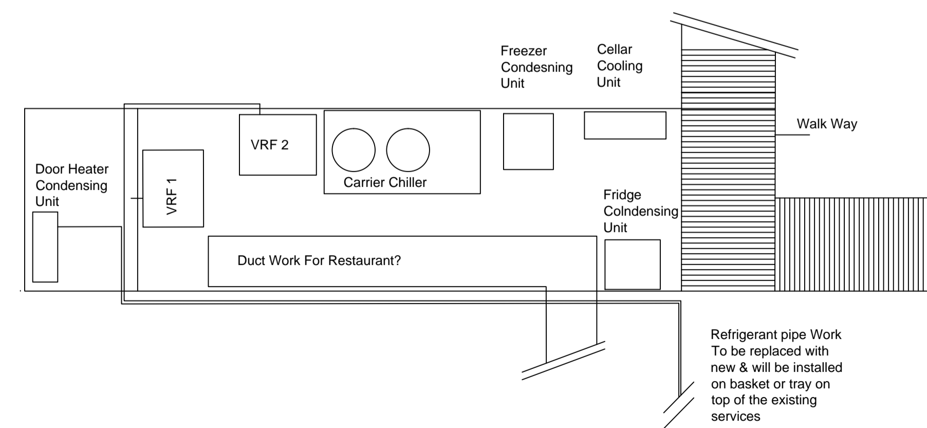
PROPOSED ROOF PLANT LAYOUT OPTION 3
