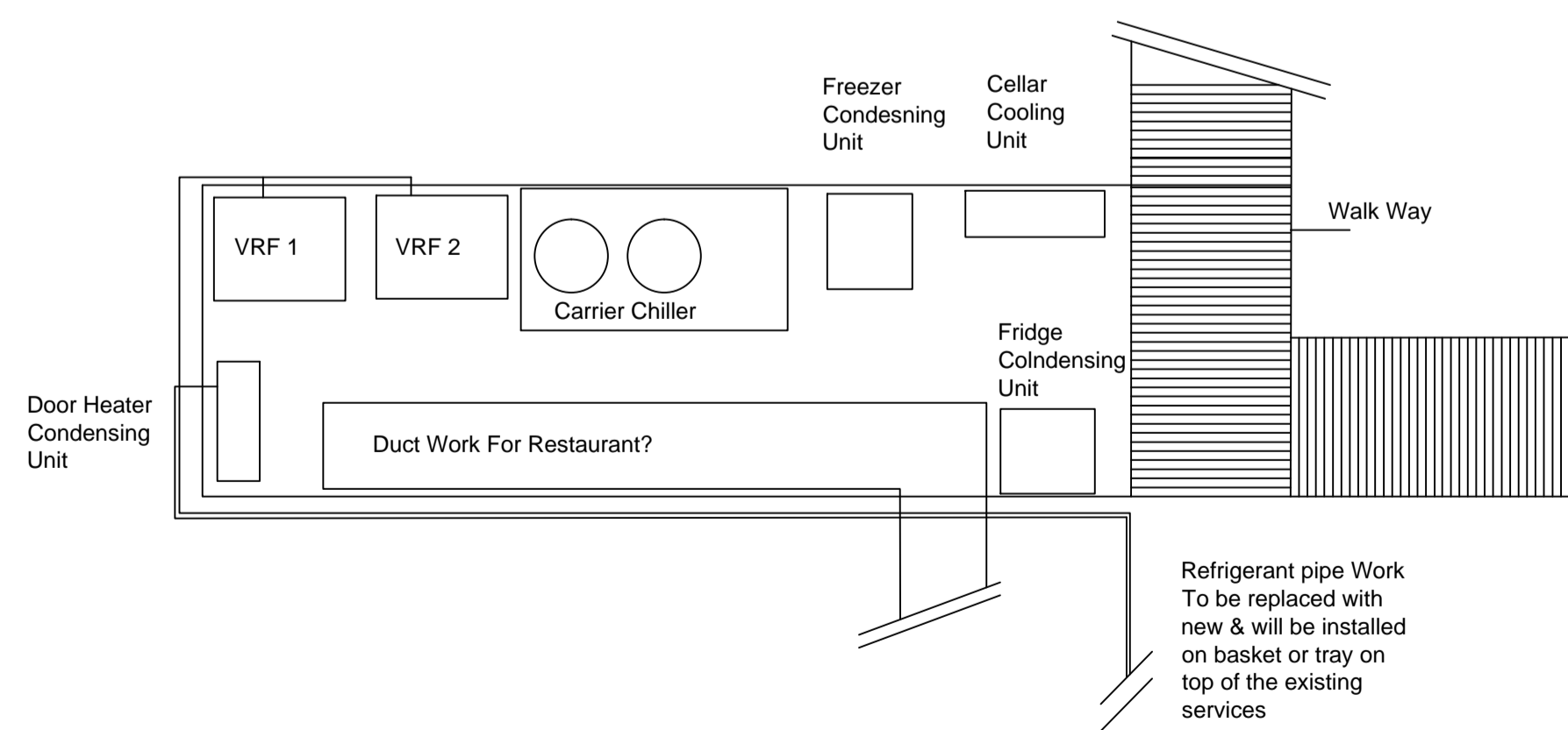
PROPOSED ROOF PLANT LAYOUT OPTION 2
