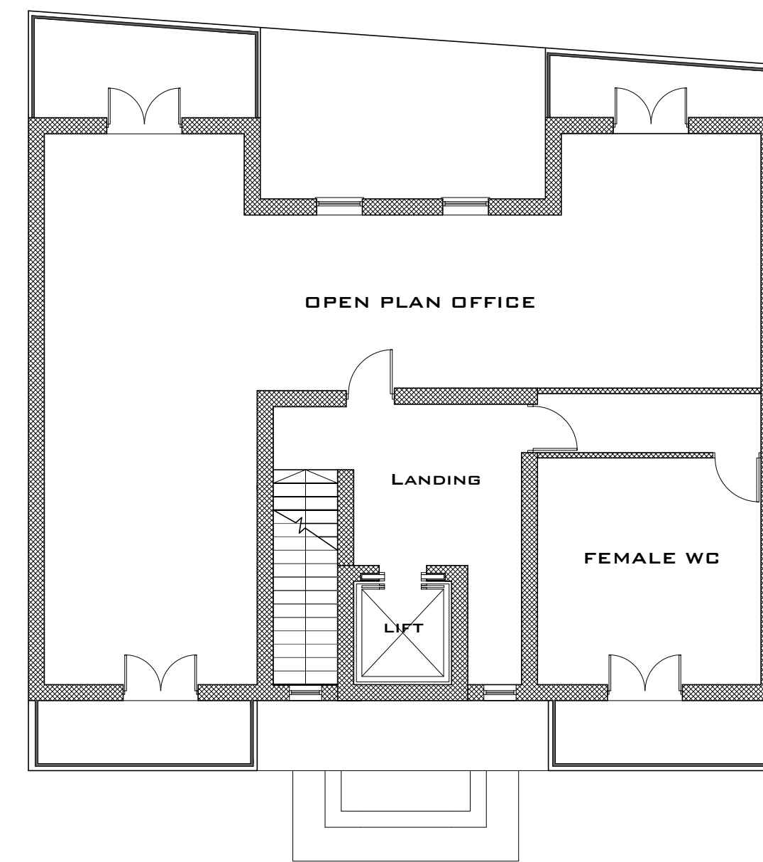
6 Proposed Fourth Floor Plan Scale: 1:100
