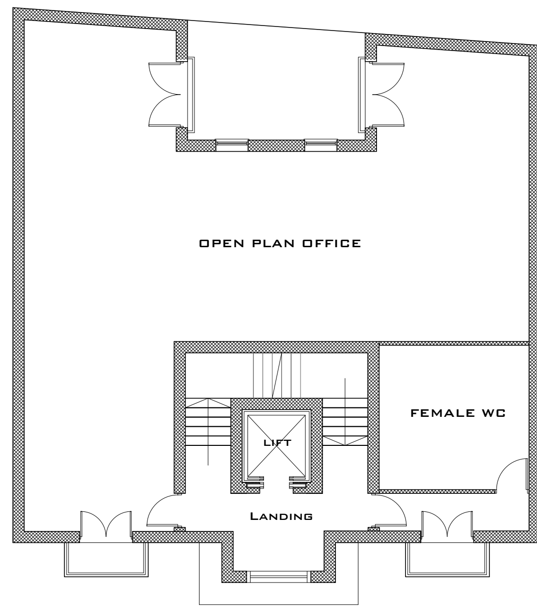
4 Proposed Second Floor Plan Scale: 1:100
