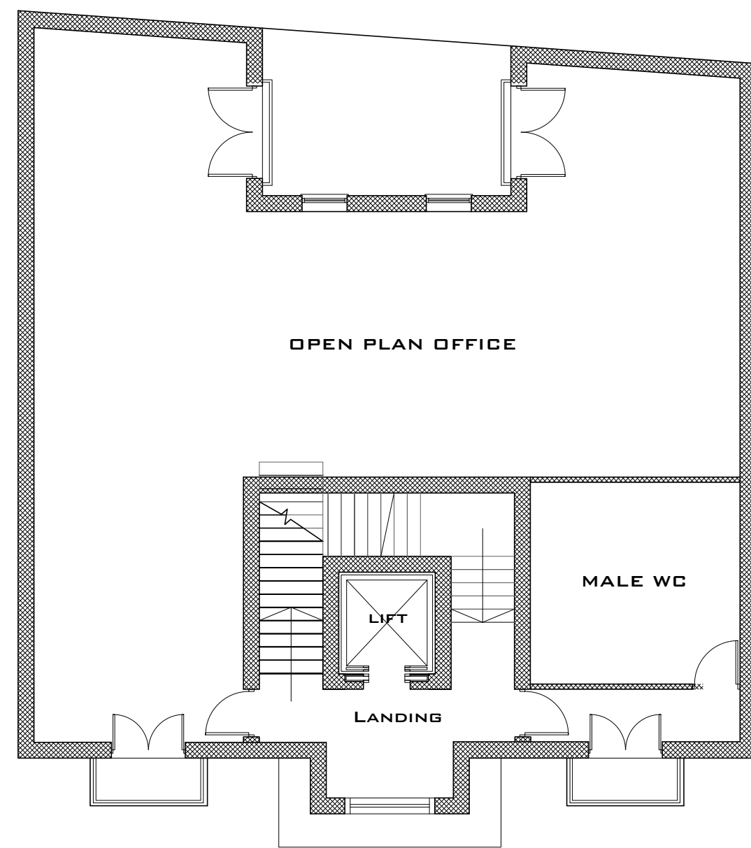
5 Proposed Third Floor Plan Scale: 1:100
