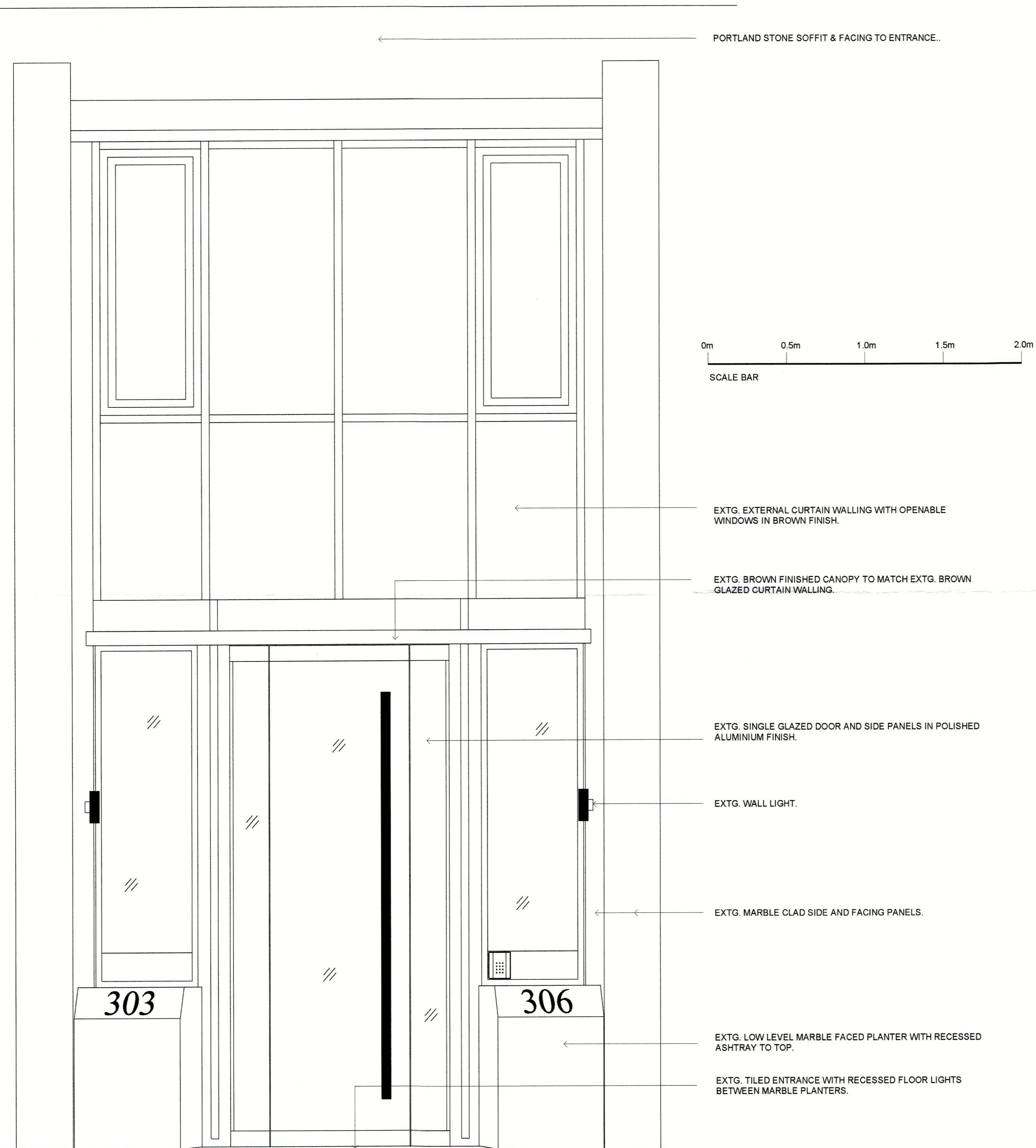
GROUND FLOOR - EXTG. ENTRANCE ELEVATION 1:20 @ A2
