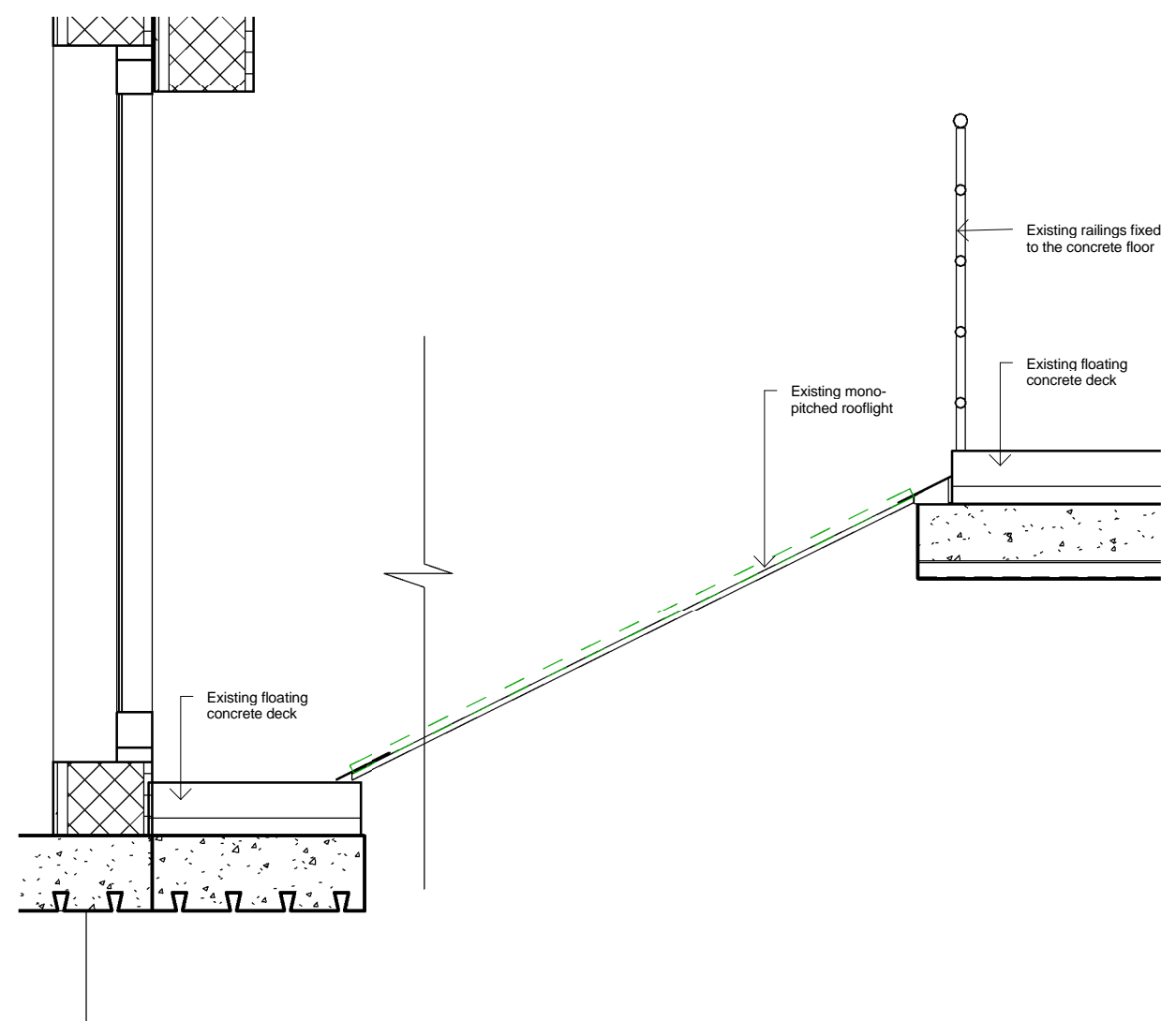
Section through existing mono-pitched glazing over Kitchen 1:20
