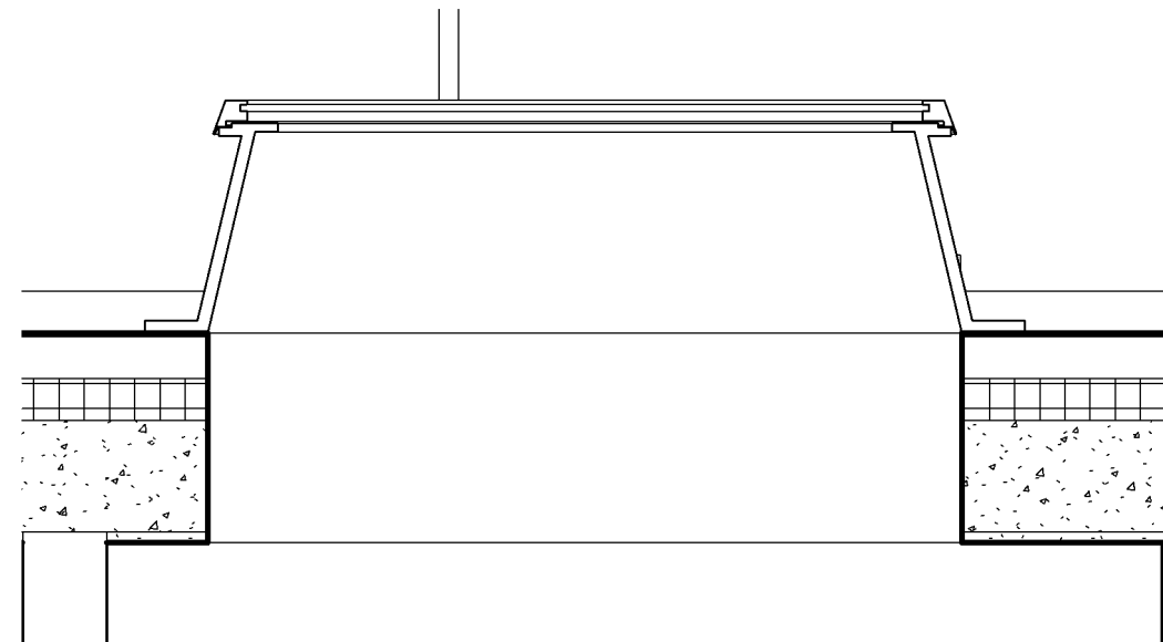
Existing Section of Typical Roof Light 1:10
