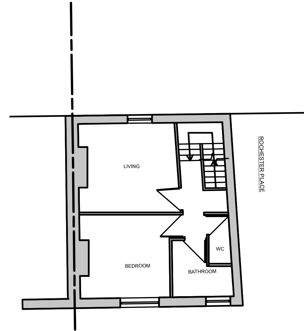
EXISTING SECOND FLOOR PLAN
