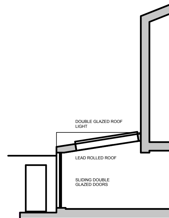
PROPOSED SECTION
