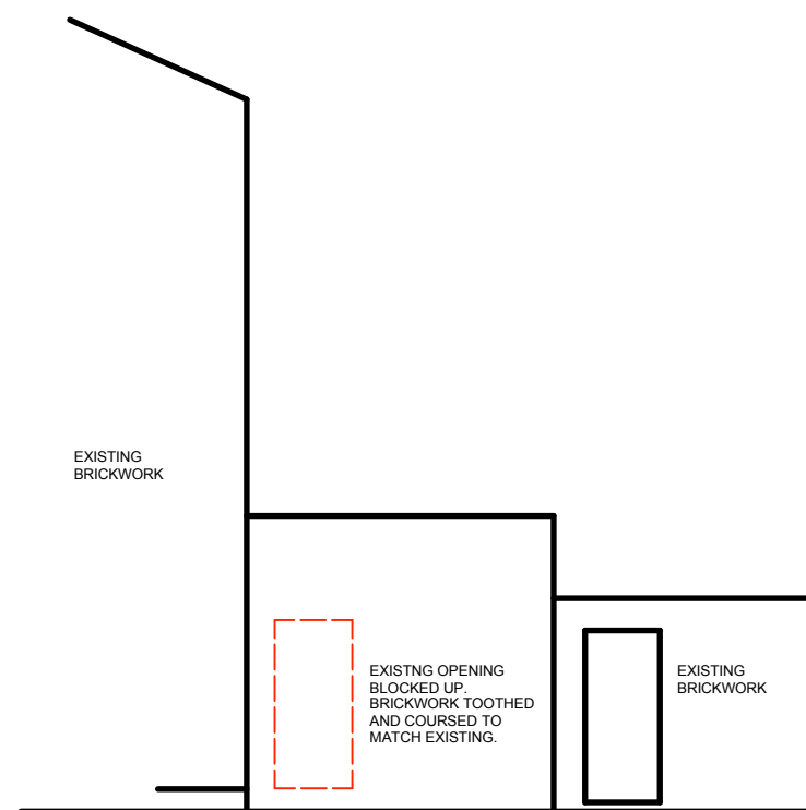
PROPOSED ELEVATION ON ROCHESTER PLACE
