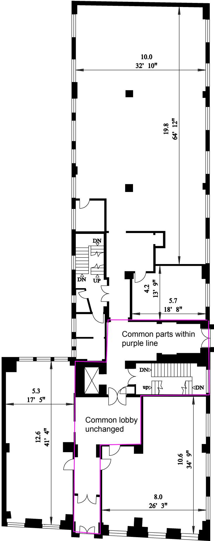
GROUND FLOOR
