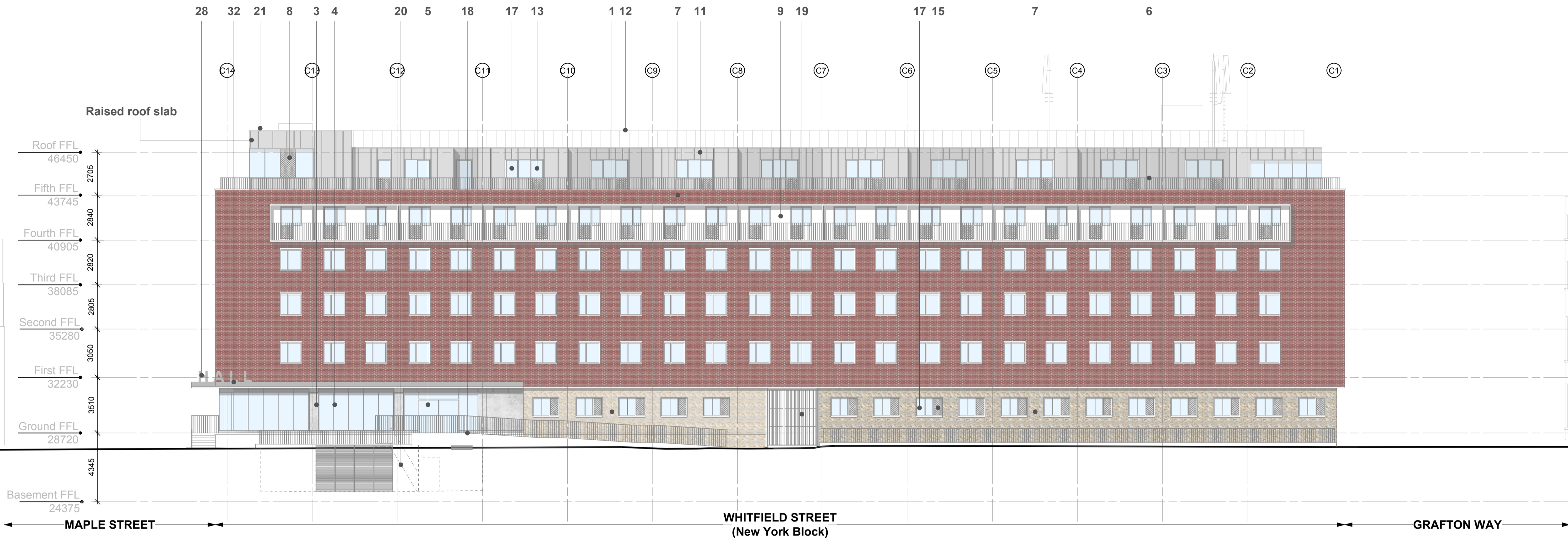
Elevation 05 New York Block Whitfield Street Elevation
