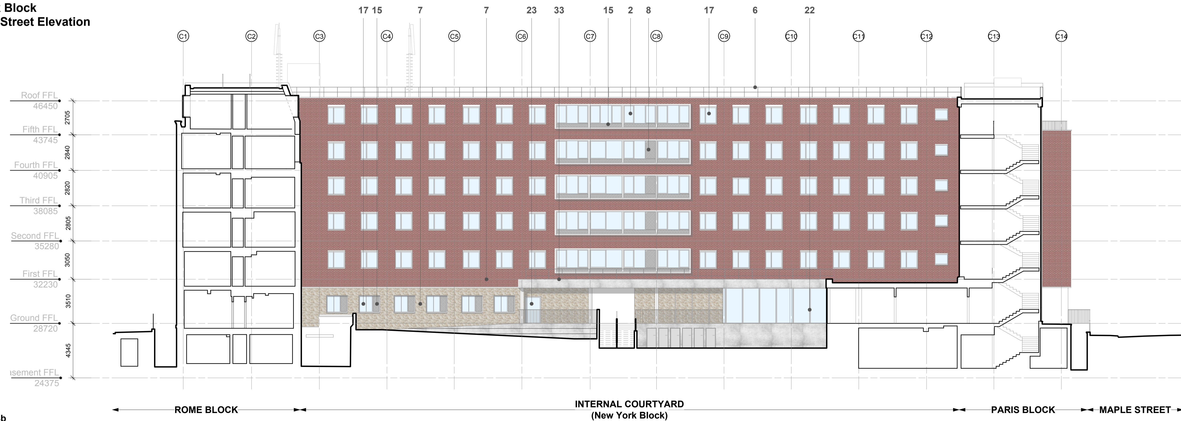
Elevation 04b New York Block Courtyard Elevation
