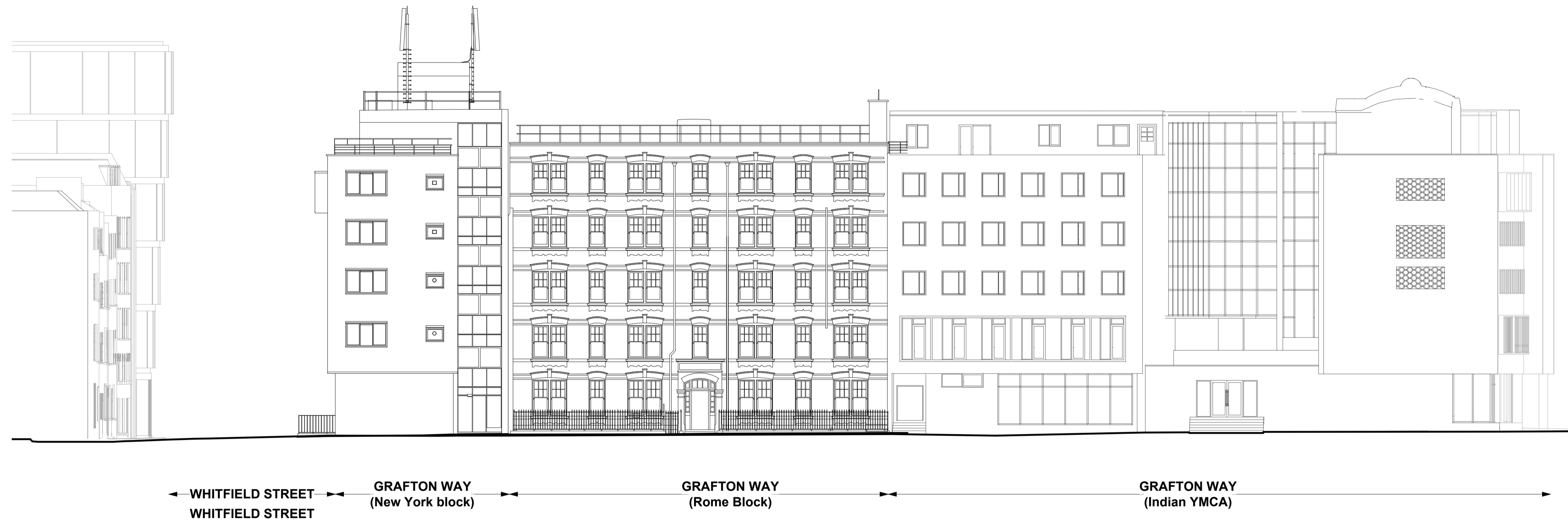
Elevation 06 Rome Block - Grafton Way Elevation
