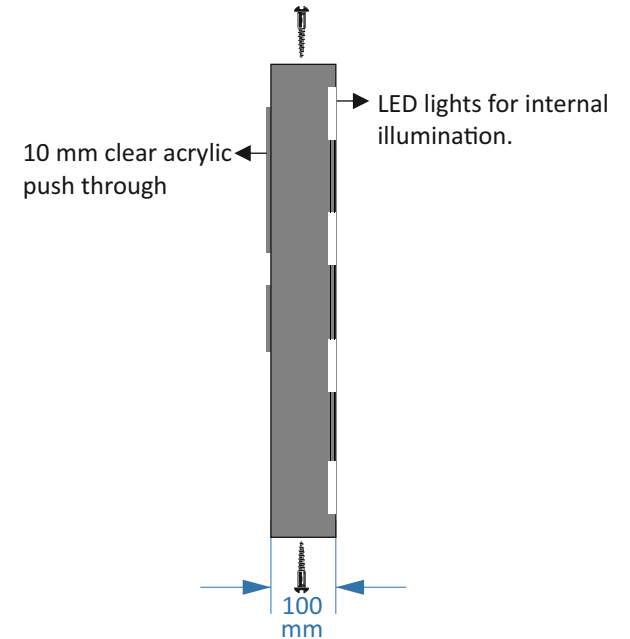
Side elevation of the main fascia sign
