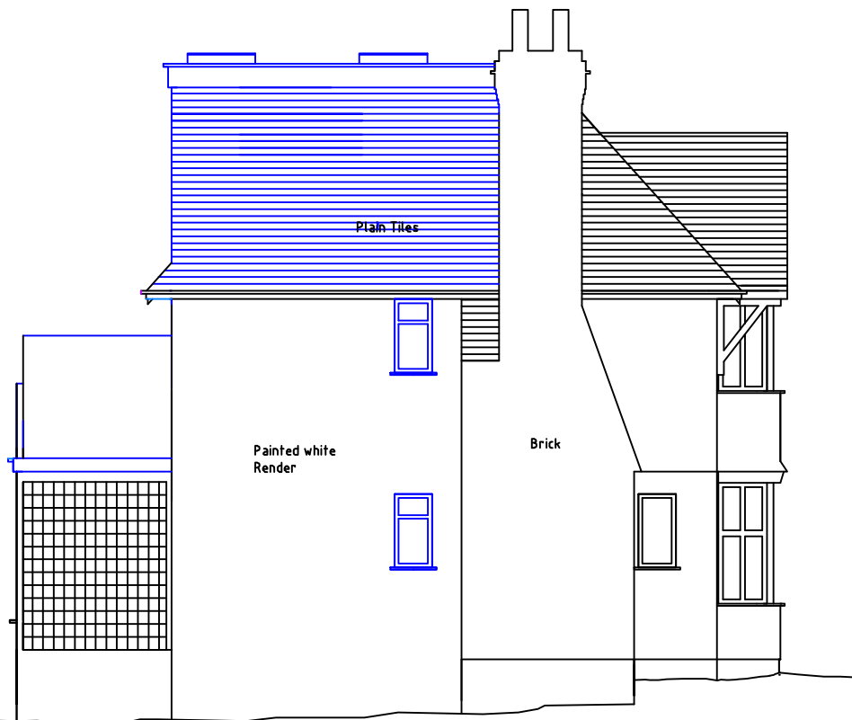
East Elevation
