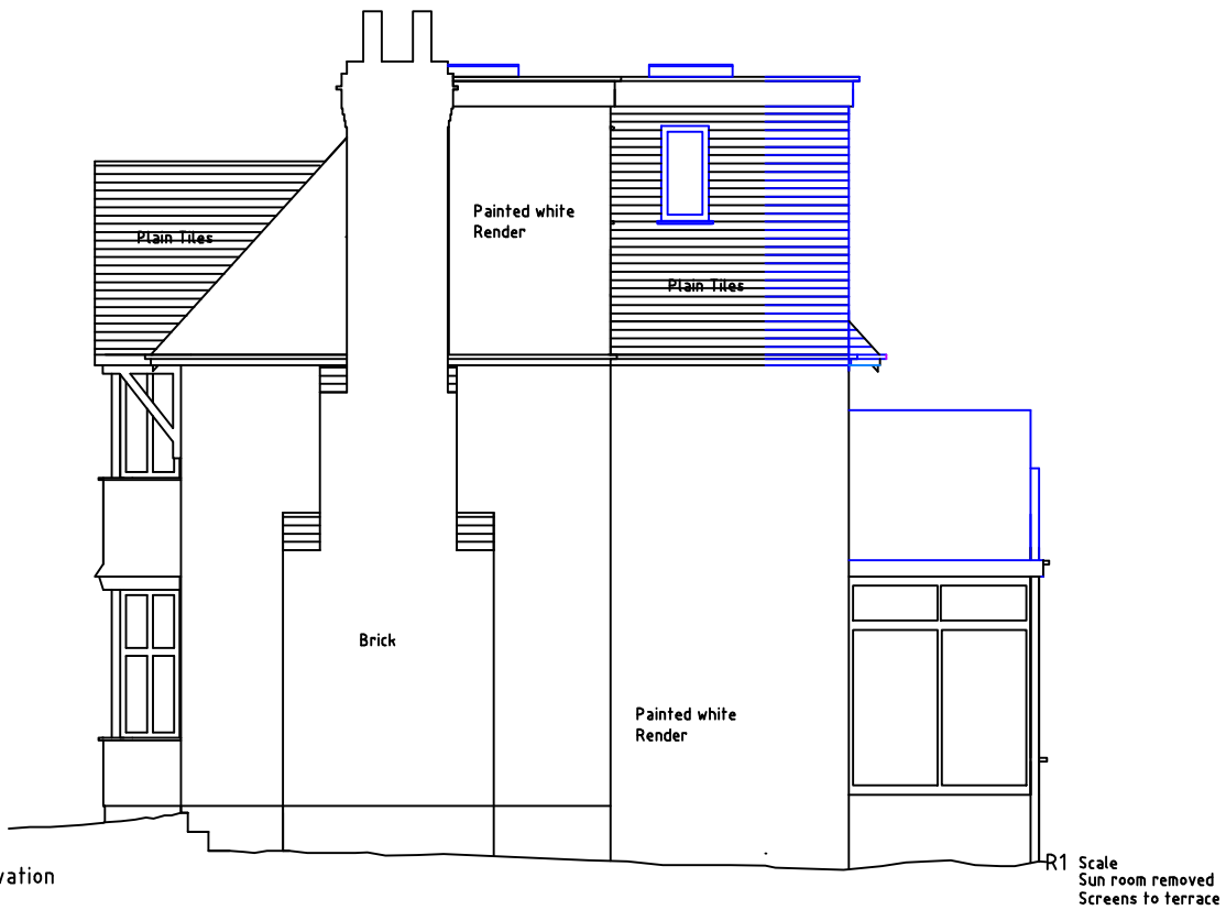
North Elevation
