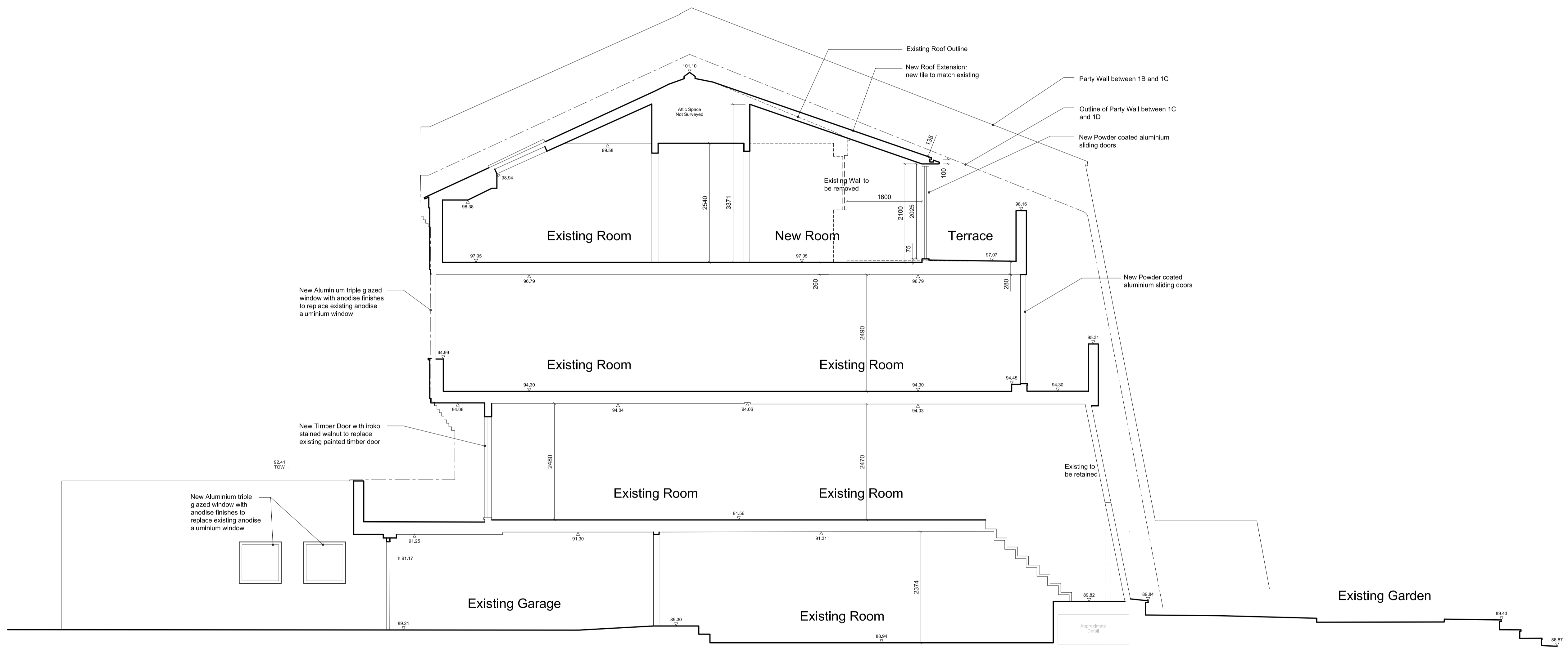
1 Proposed Section B 0 1 3m
