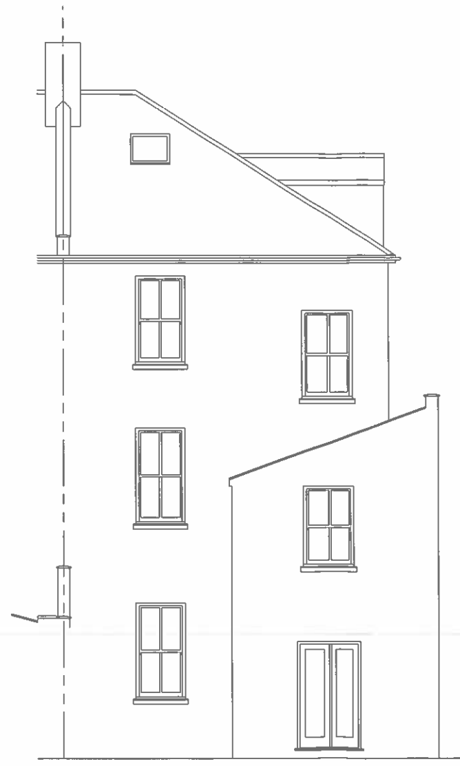
REAR ELEVATION
