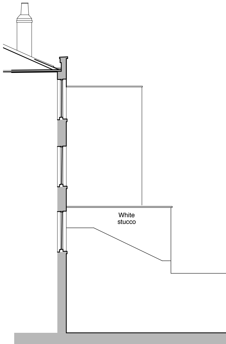
LEFT REAR ELEVATION
