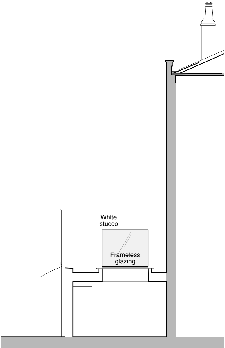
RIGHT REAR ELEVATION
